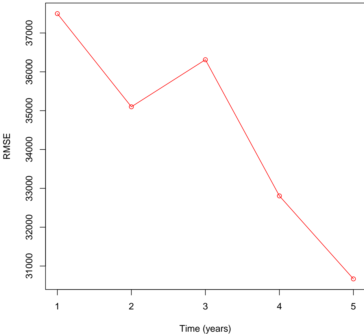
RMSE of ice thickness over time for sample2
