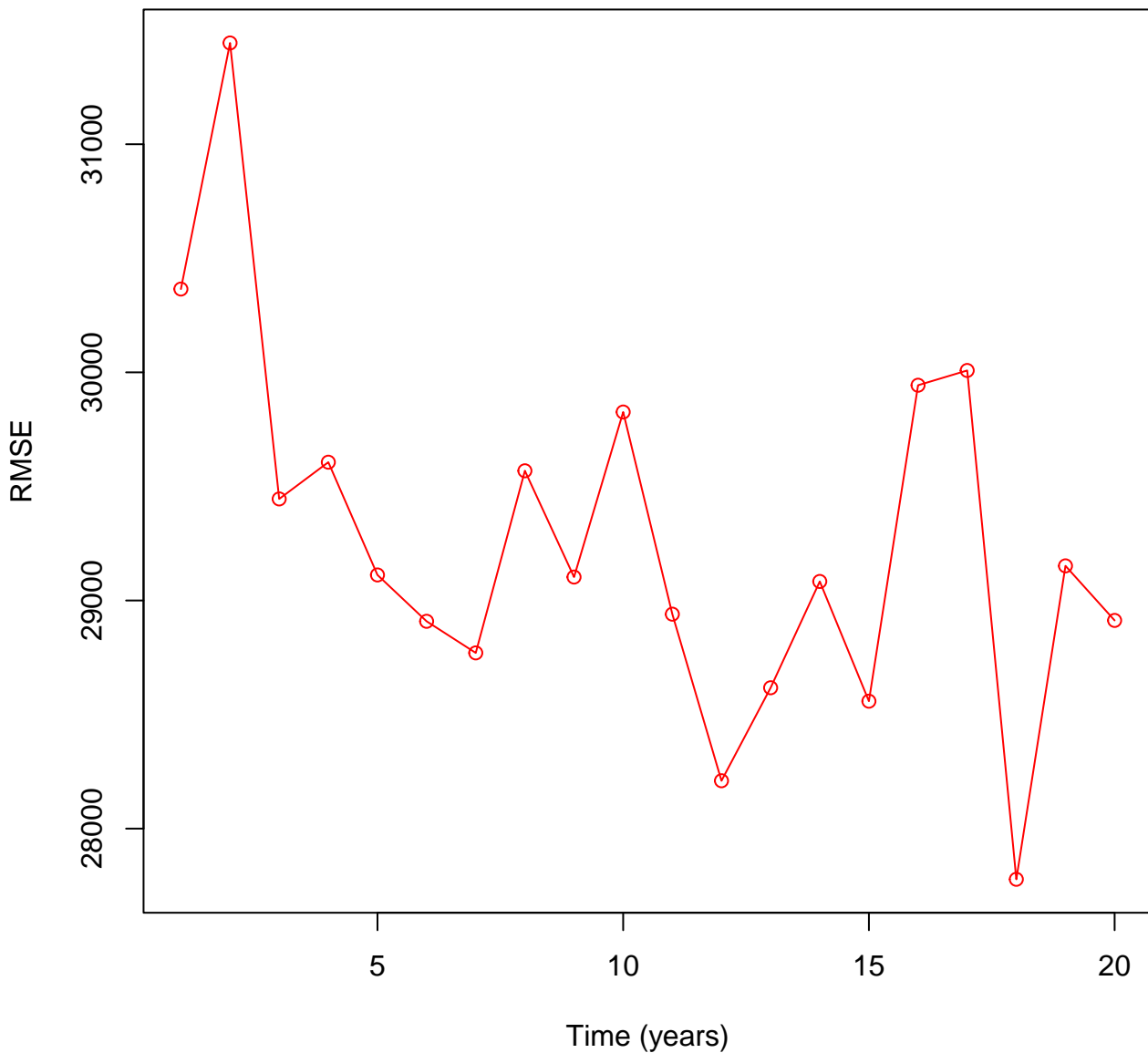
RMSE of ice thickness over time for sample3
