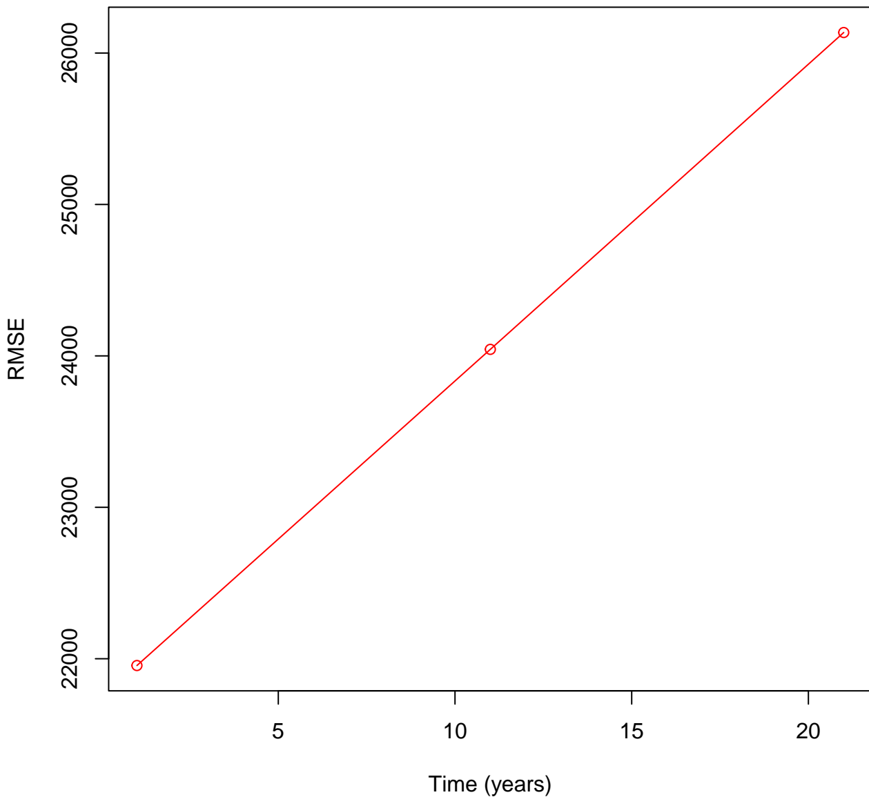
RMSE of ice thickness over time for sample37
