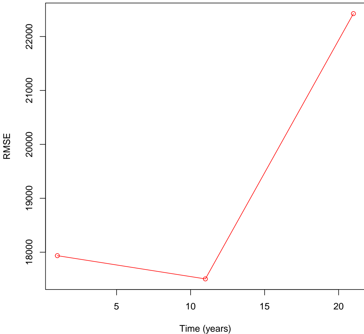
RMSE of ice thickness over time for sample15
