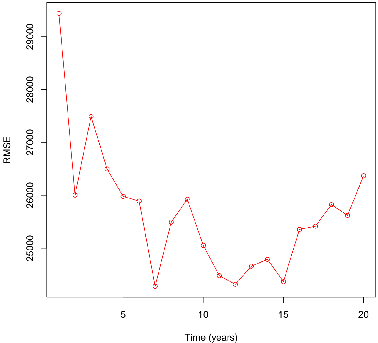
RMSE of ice thickness over time for sample1
