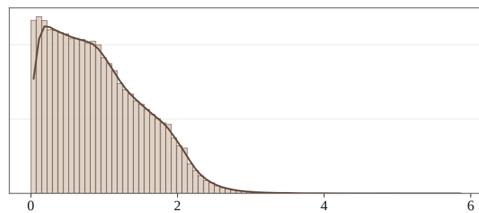
Rating residual
