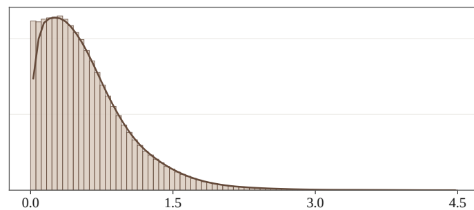
Absolute residual
