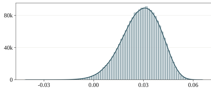
Decision-function score
