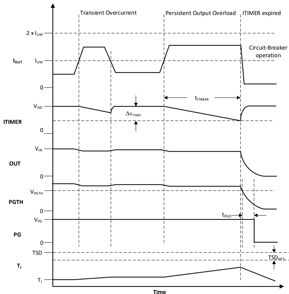
Figure 8-9. TPS259474x Overcurrent Response
