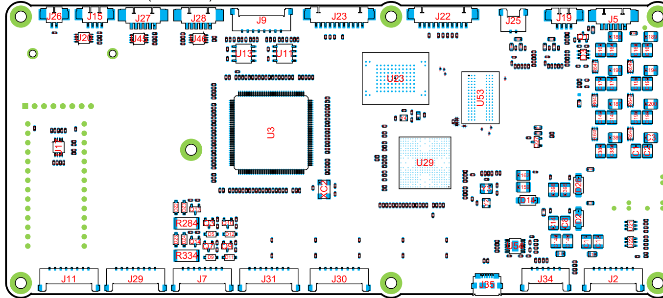
View from Bottom side (Scale 1:1)
