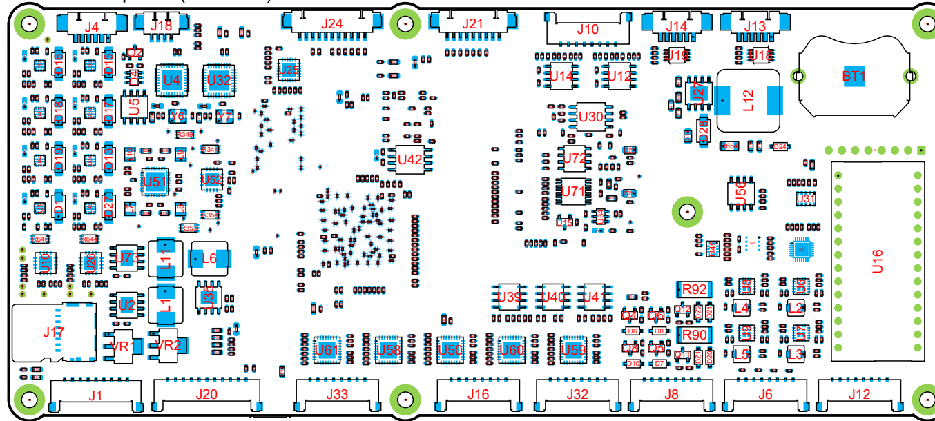
View from Top side (Scale 1:1)
