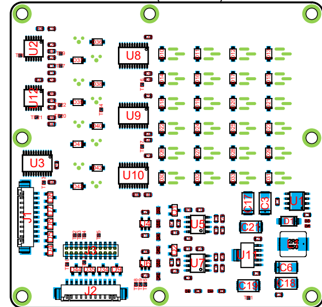
View from Bottom side (Scale 1:1)
