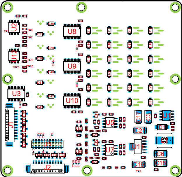
View from Bottom side (Scale 1:1)
