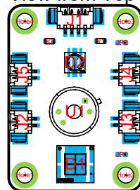
View from Top side (Scale 1:1)
