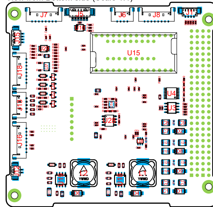
View from Bottom side (Scale 1:1)
