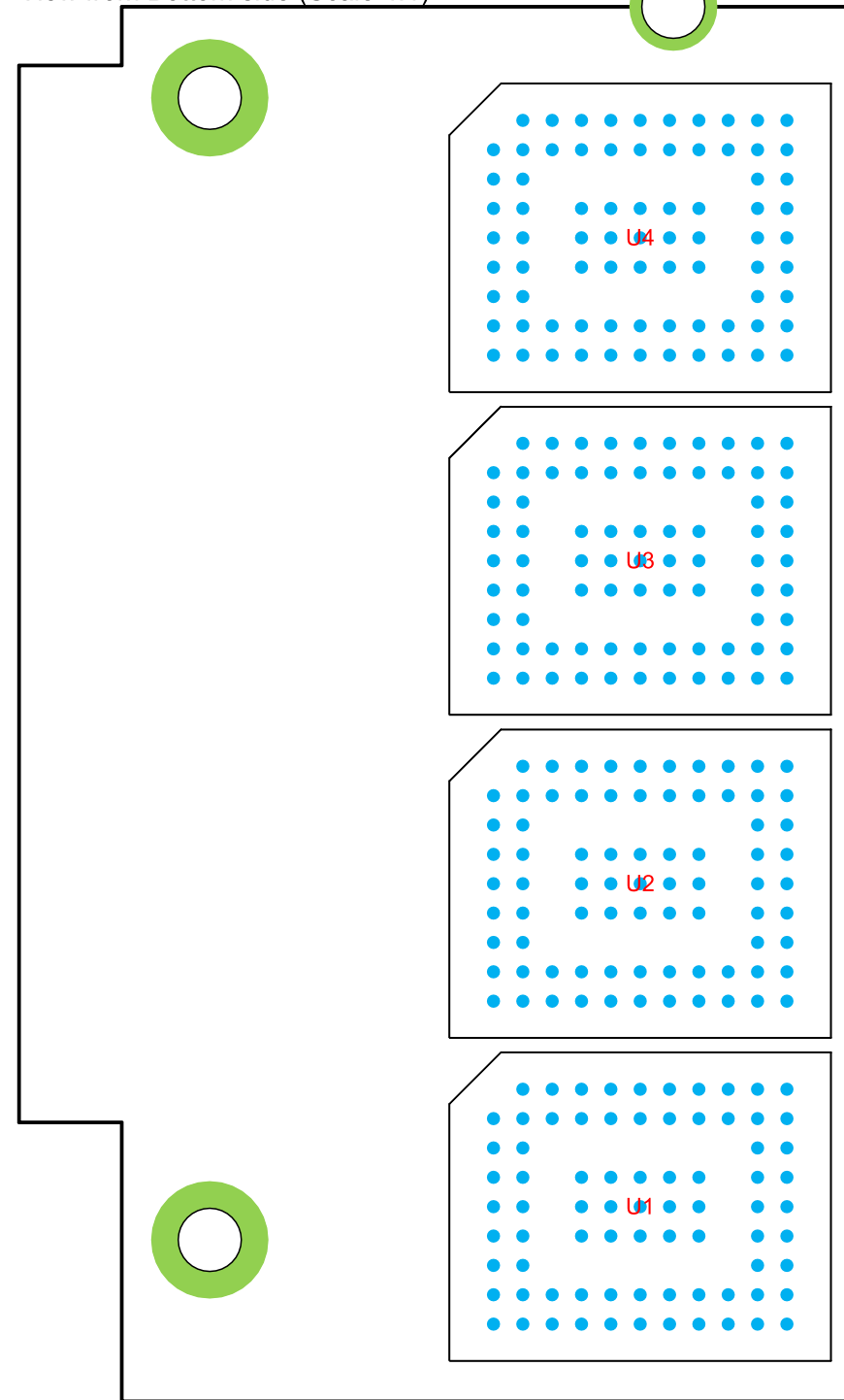
View from Bottom side (Scale 4:1)
