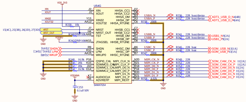
MPU configuration
