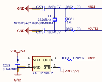
32.768KHz clock
