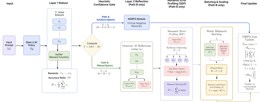
Fig. 1. The complete system architecture of SB-GRPO. The Heuristic Confidence Gate ( \Gamma ) dynamically routes uniform batches to the NGRPO module (Path A) to prevent advantage vanishing. For mixed batches (Path B), the framework applies Multi-Layer Reflection and Semantic Error Profiling (SEP) to extract the Top Error Cluster ( C_{top} ), forming a Static Balanced Batch optimized by an Entropy-Aware Loss Scaling factor ( \lambda ).
