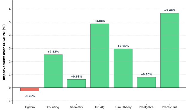
Figure 1: Relative performance gain of H-MSB-GRPO compared to the M-GRPO baseline. The significant improvements in Intermediate Algebra (+4.88%) and Precalculus (+5.68%) demonstrate the effectiveness of semantic balancing in complex reasoning, while the stability in Algebra confirms that the Heuristic Confidence Gate prevents correction bias in simpler tasks.
