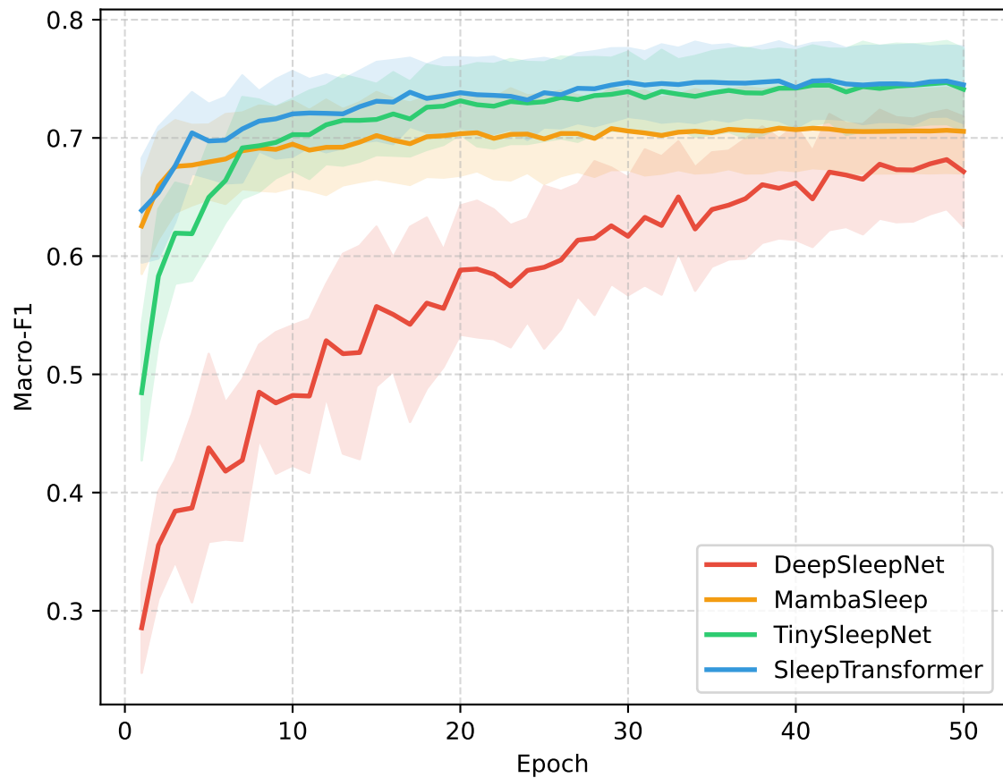
Validation Macro-F1 across 10 Folds
