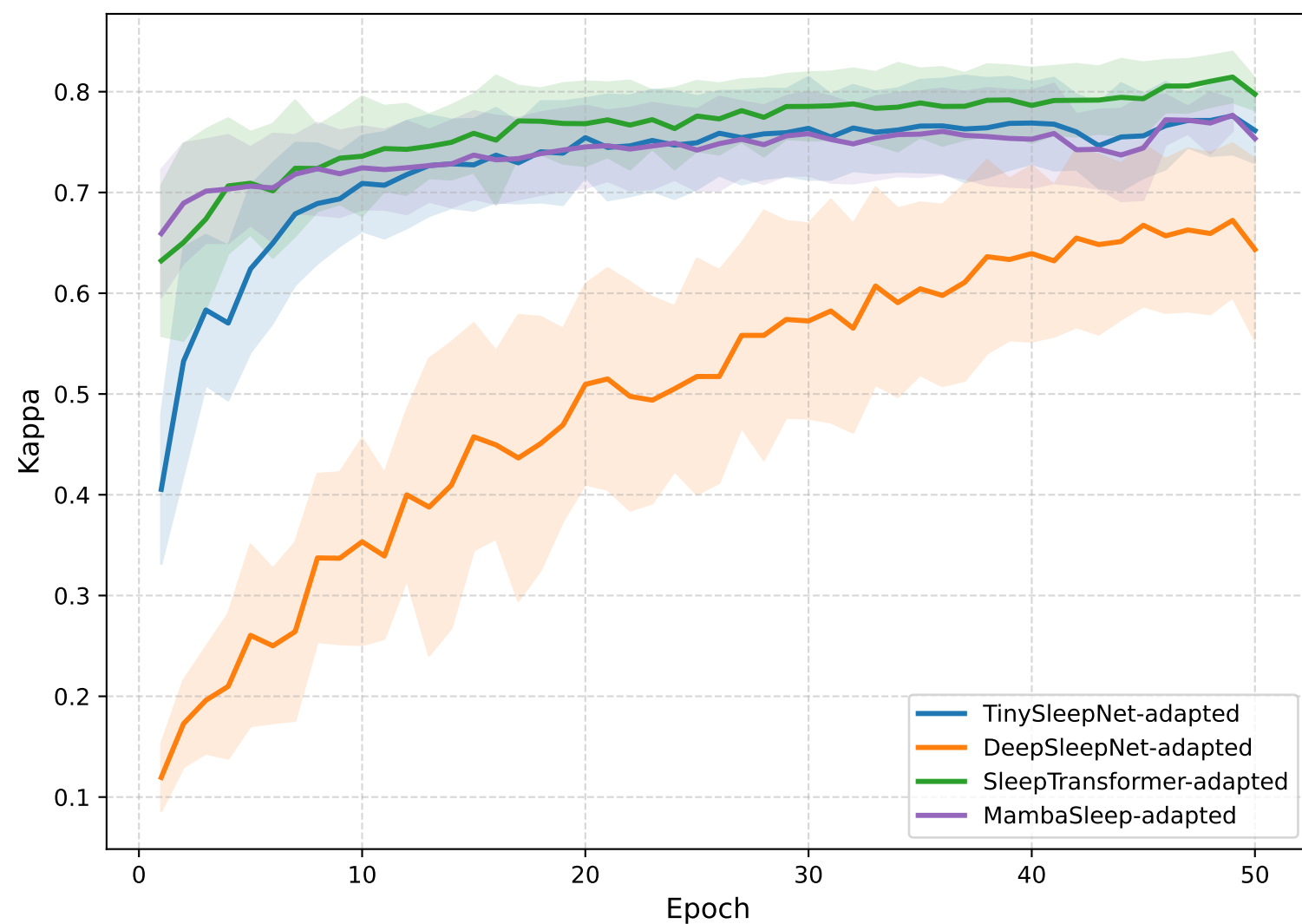
Validation Cohen's Kappa
