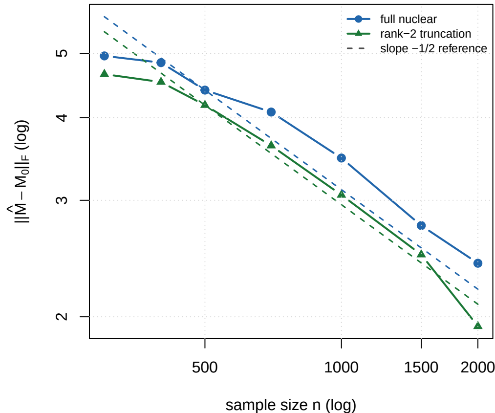
Log-log slopes: full -0.396, rank -0.464
