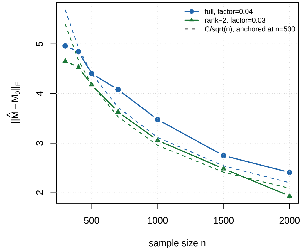
Nuclear Frobenius error
