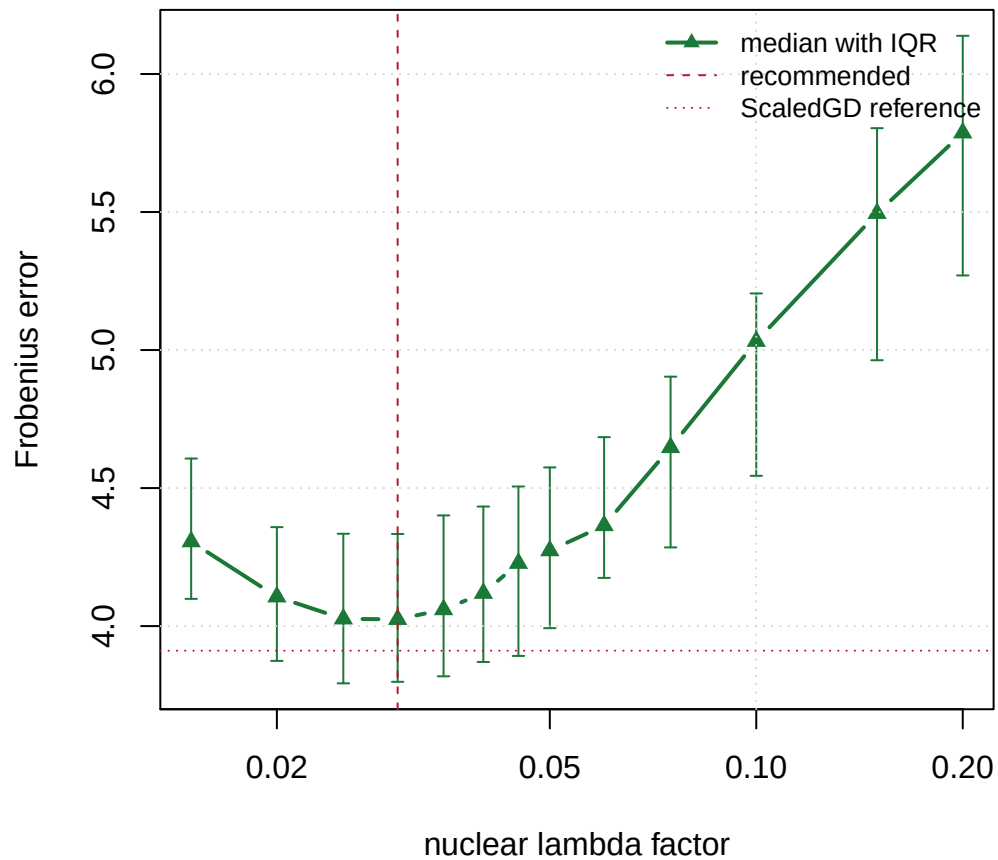
After rank-2 truncation
