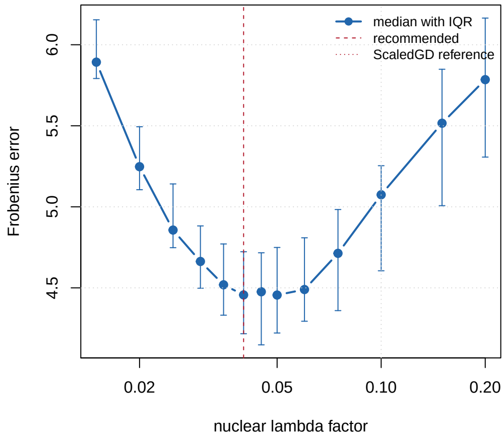
Full nuclear estimate
