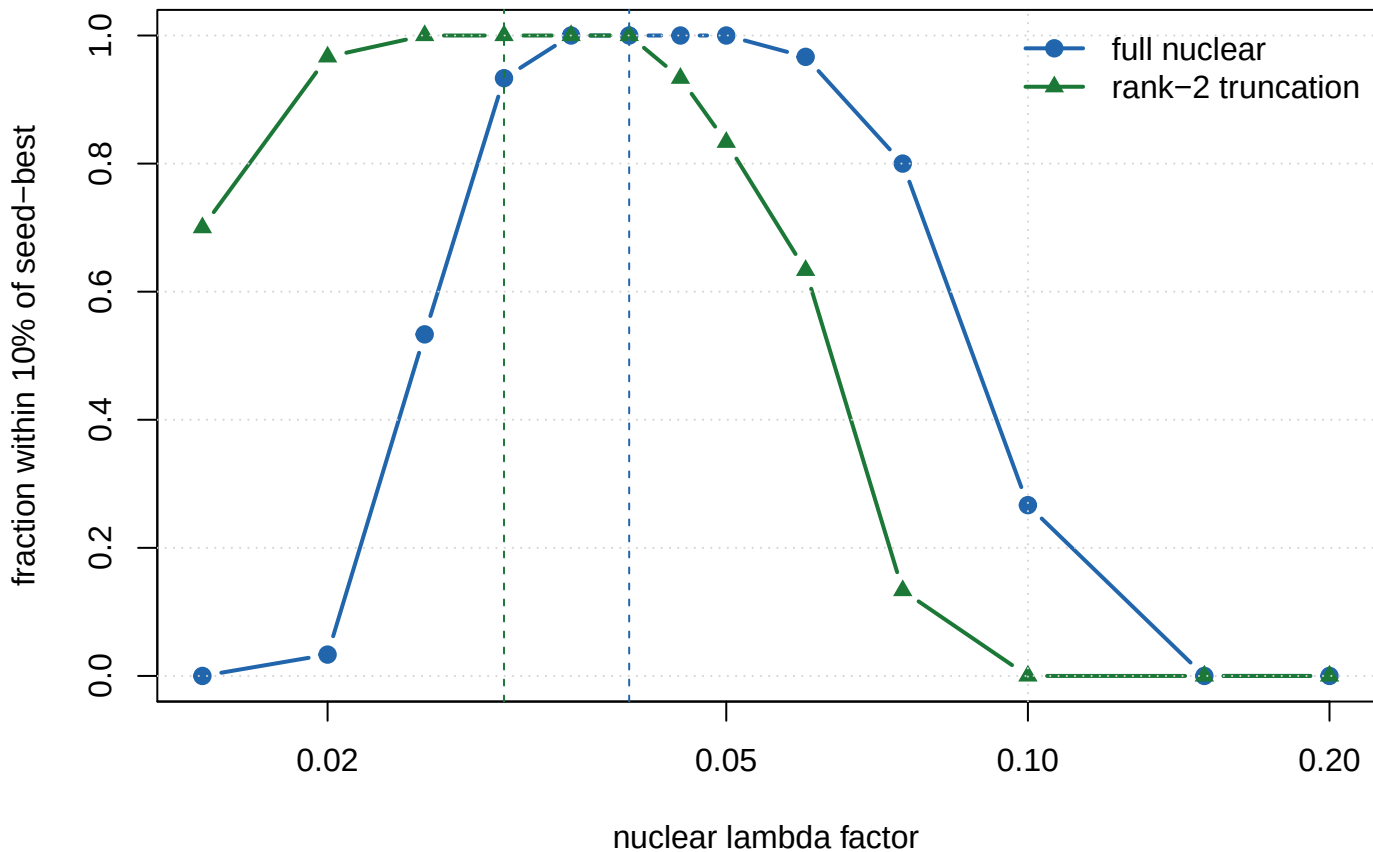
Near-best frequency across seeds
