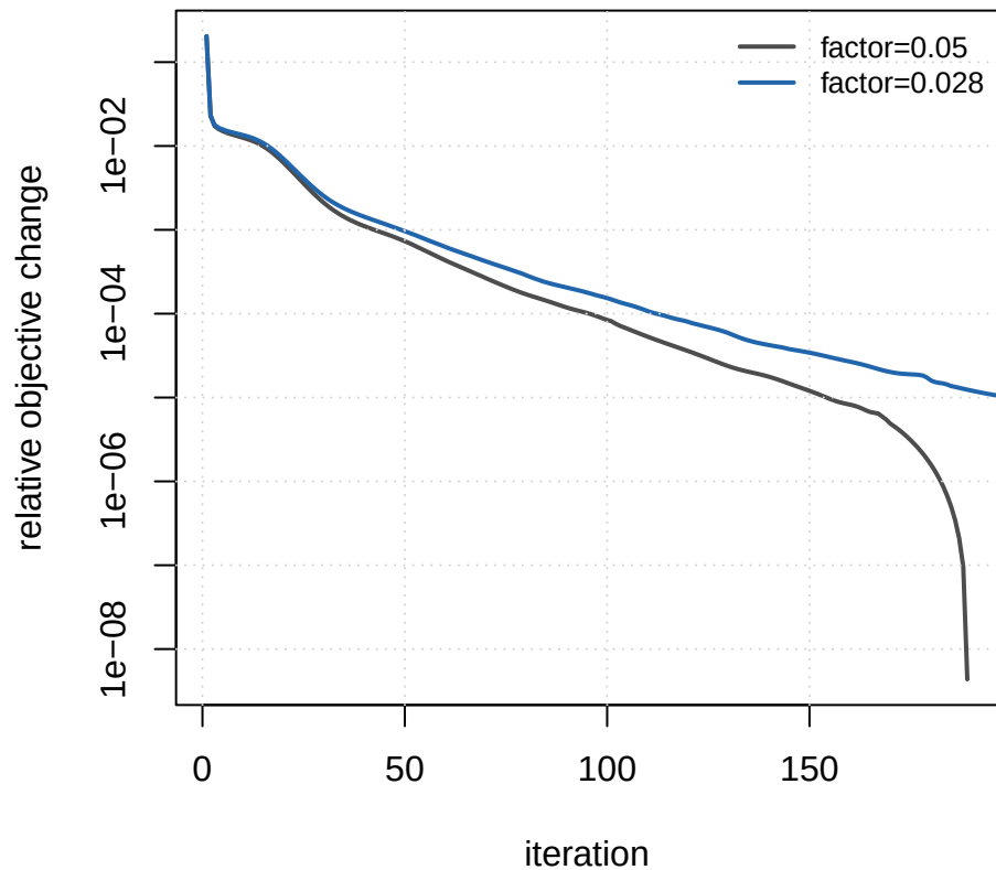
Objective-change stopping metric
