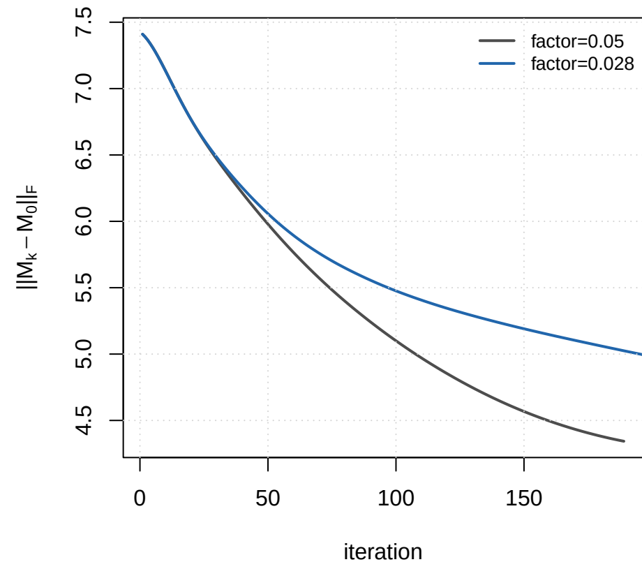
Truth Frobenius trajectory
