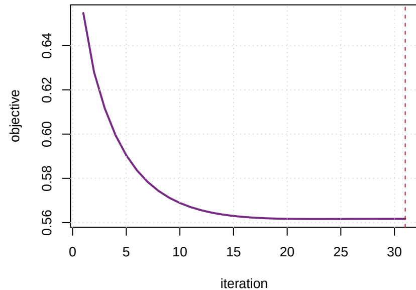
Penalized objective
