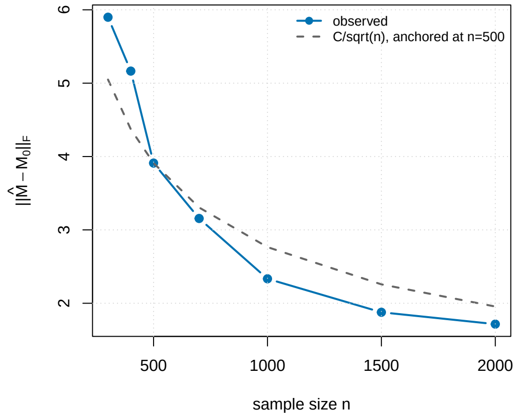
Frobenius error, n=300–2000
