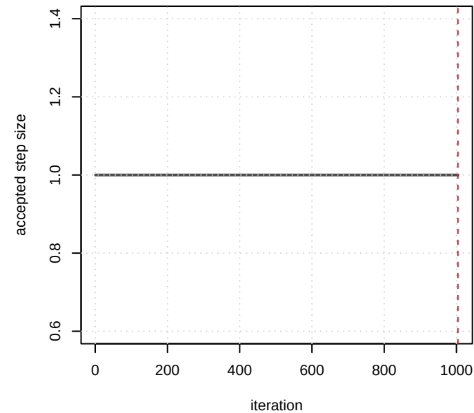
Backtracking step size
