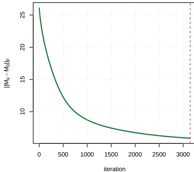
Backtracking step size
