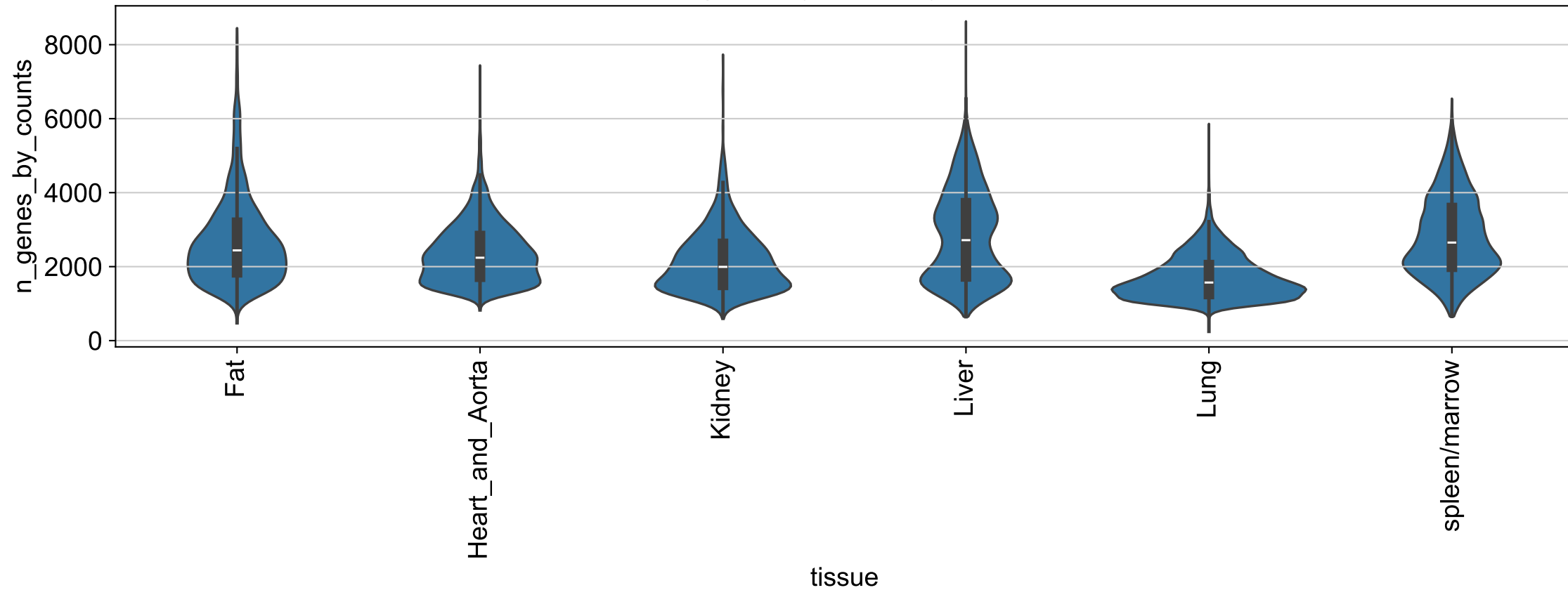
n_genes_by_counts by tissue
