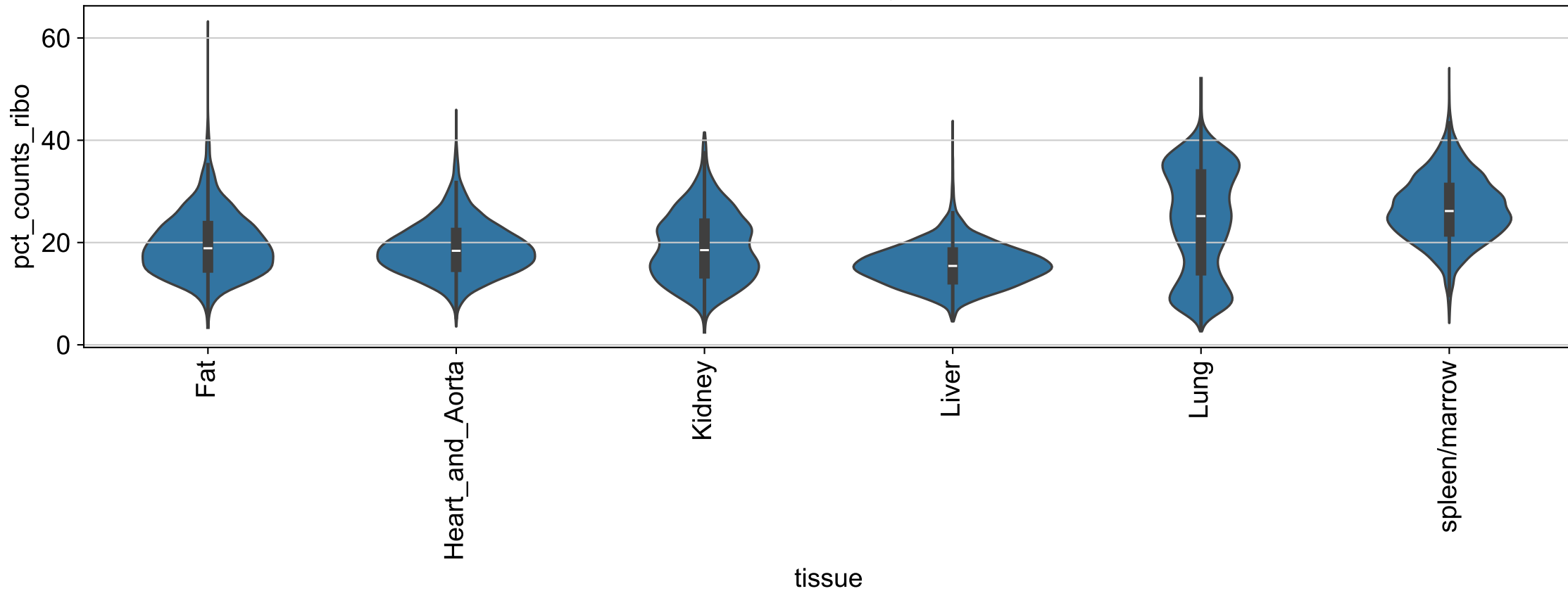
pct_counts_ribo by tissue
