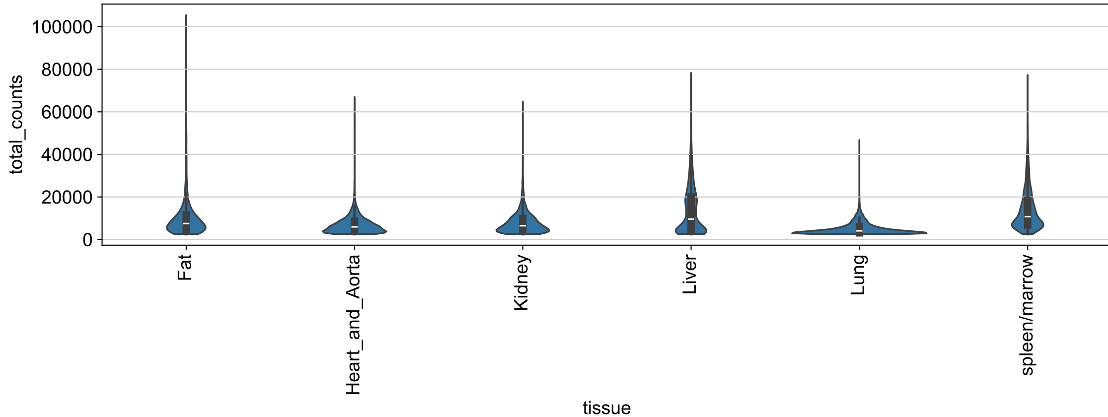
total_counts by tissue
