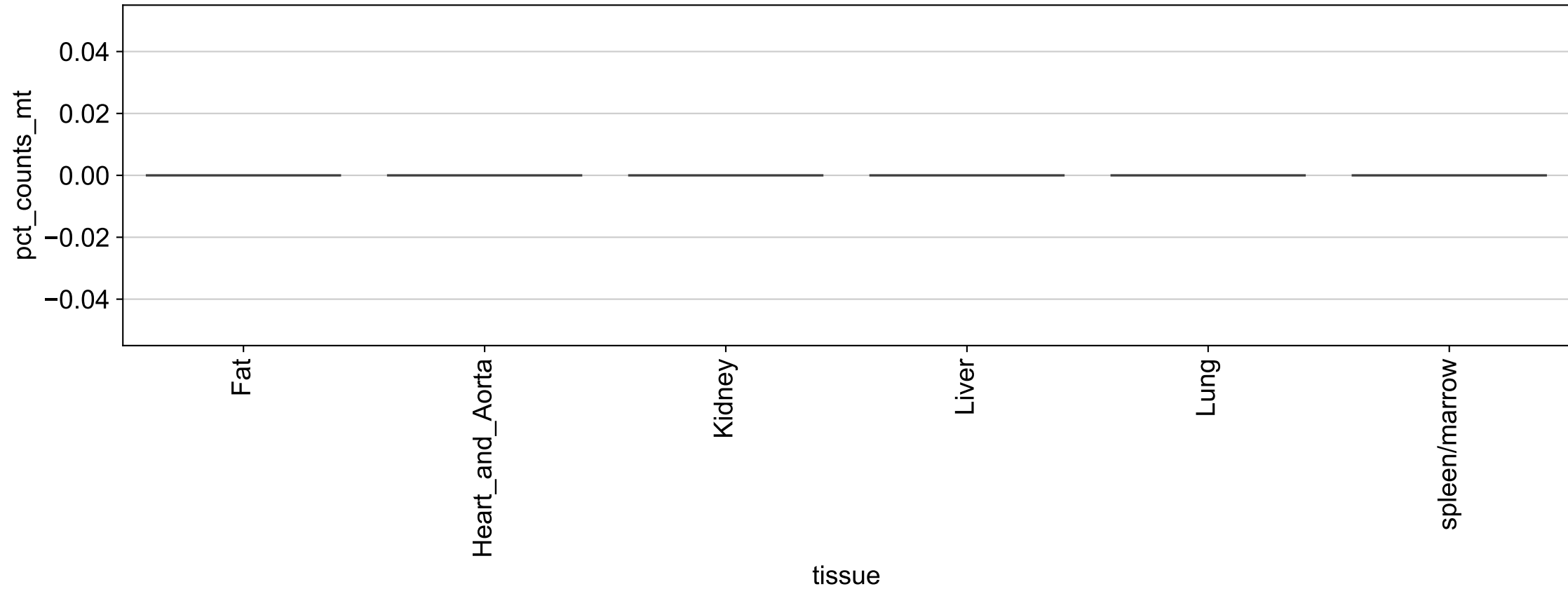
pct_counts_mt by tissue
