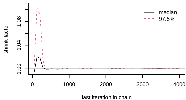
gamma[7,3]
