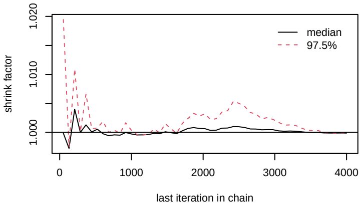
lambda0[6]
