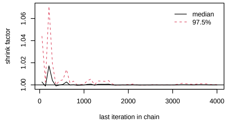
lambda0[7]
