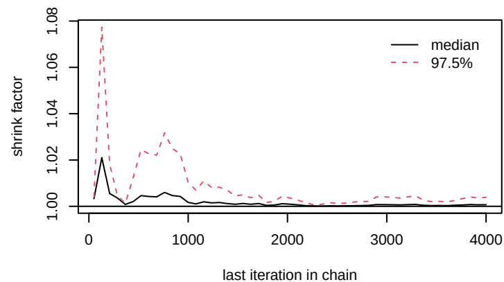
gamma[4,2]
