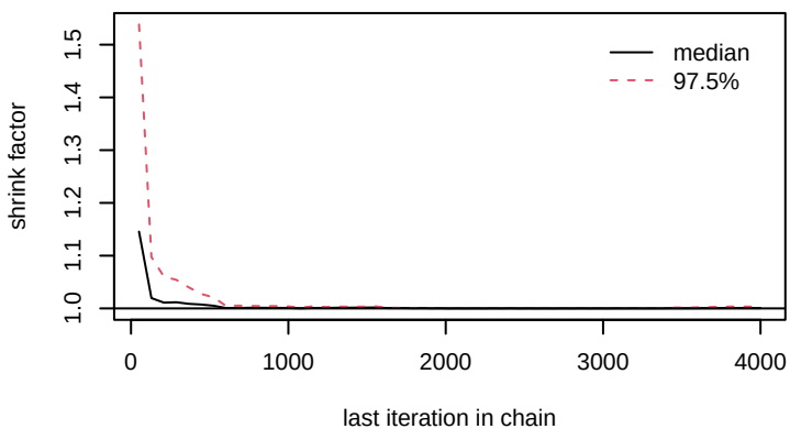
gamma[9,6]
