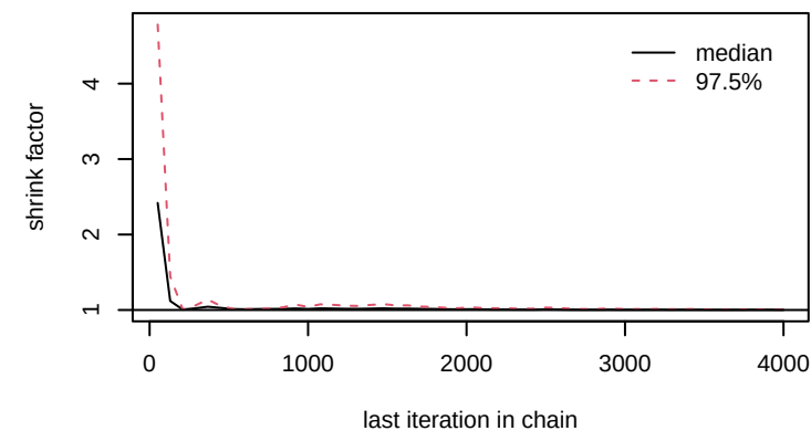
beta_long[5]
