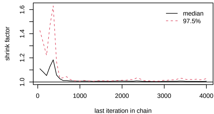
alpha1[8]
