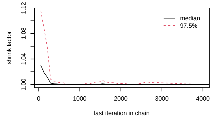
gamma[2,8]
