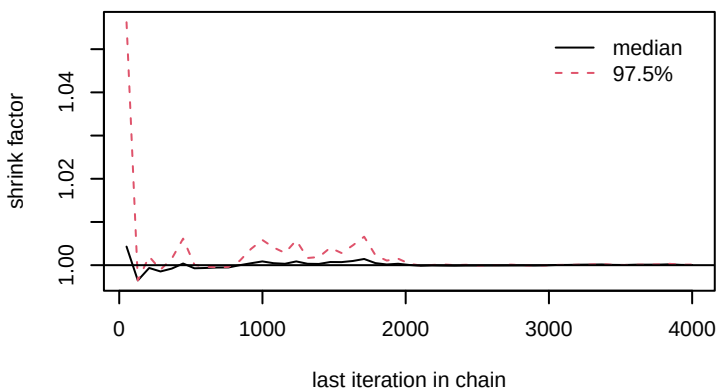
gamma[6,3]
