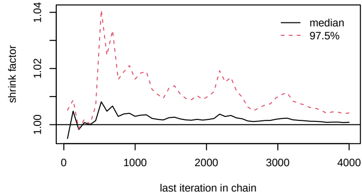
lambda0[4]
