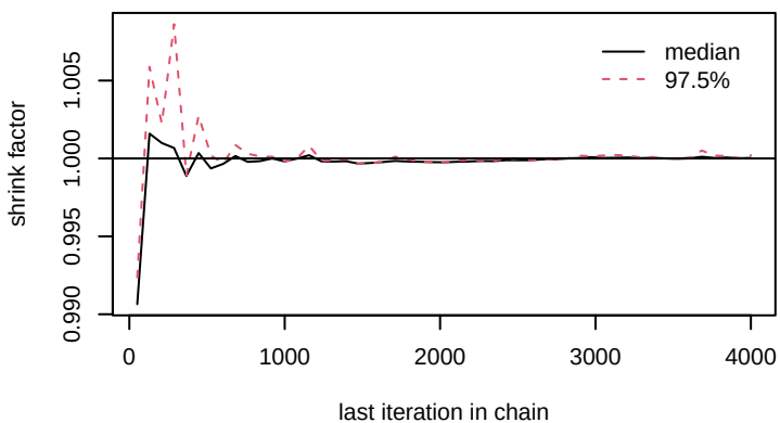
gamma[9,3]
