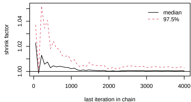
gamma[7,2]
