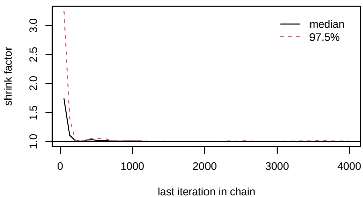
beta_long[3]
