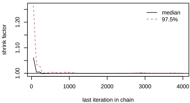
gamma[9,4]
