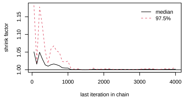
alpha1[2]
