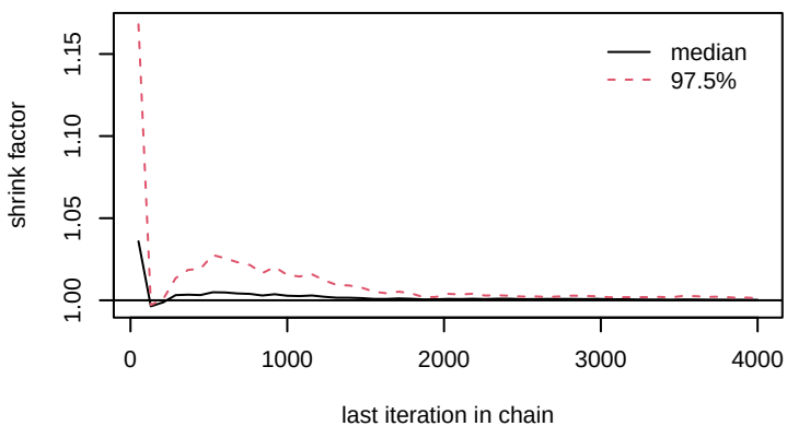
gamma[6,4]
