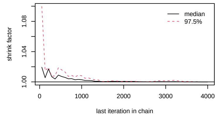
gamma[2,2]
