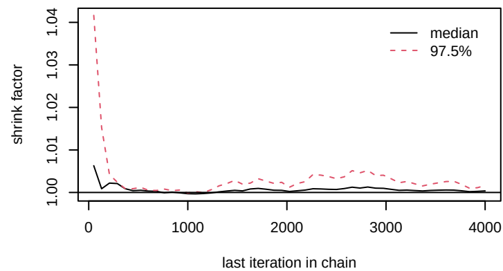
gamma[1,5]
