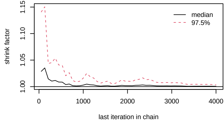
gamma[4,3]
