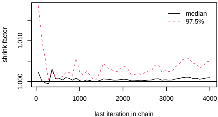
gamma[3,8]
