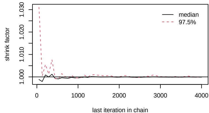
gamma[4,6]
