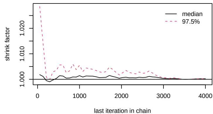
gamma[7,5]
