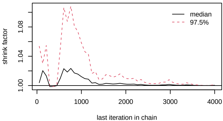
alpha1[7]
