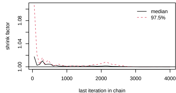
gamma[5,7]
