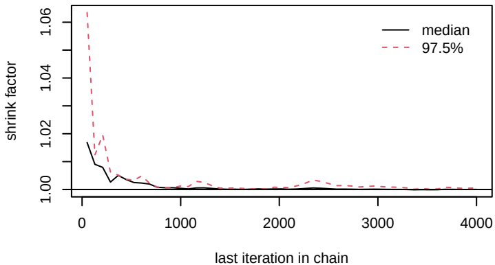
gamma[9,7]
