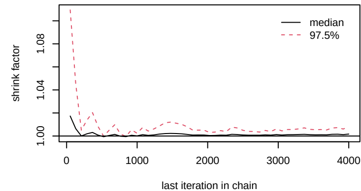
gamma[8,1]
