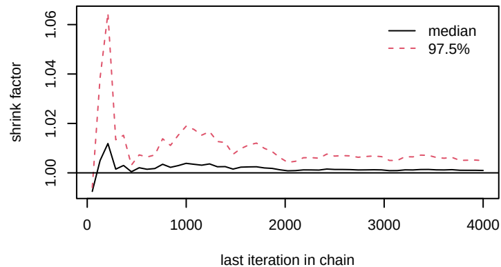
gamma[4,8]
