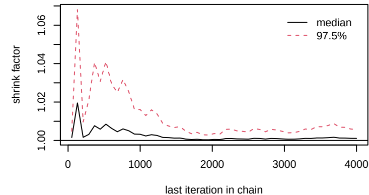
gamma[5,8]
