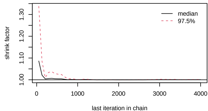
gamma[4,7]
