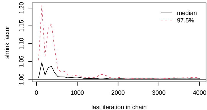
sigma_y
