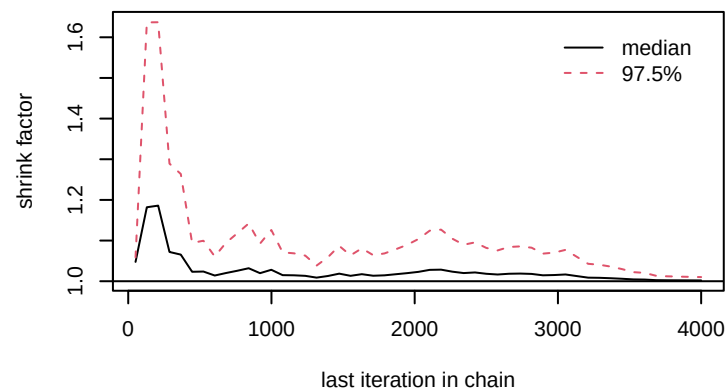
beta_long[4]
