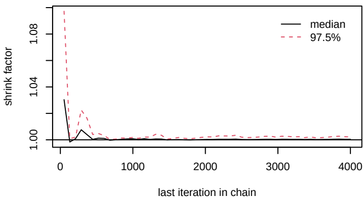
gamma[3,5]
