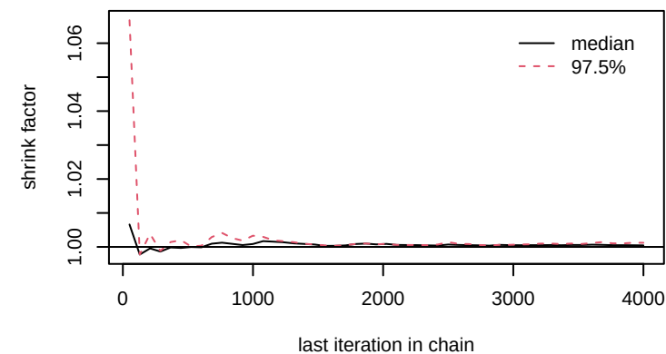
gamma[2,1]
