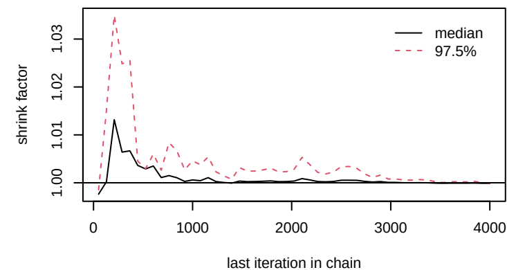
gamma[8,7]
