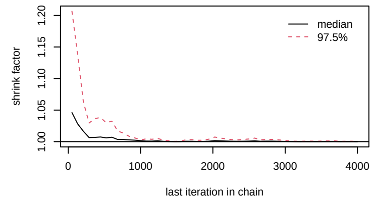
alpha0[6]
