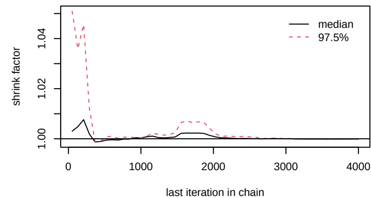
gamma[8,6]
