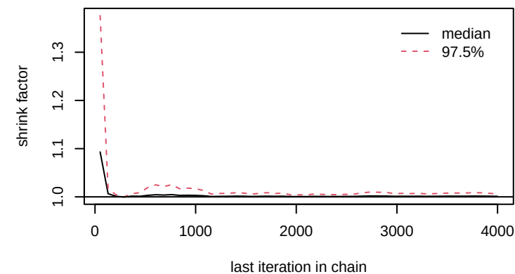
gamma[2,6]
