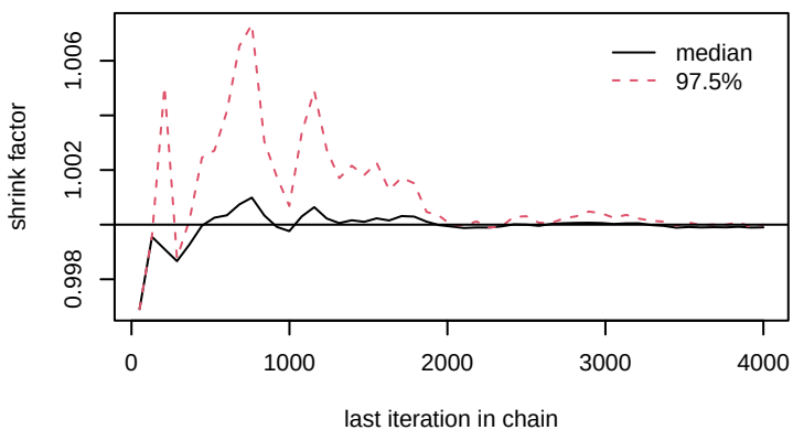
gamma[6,2]
