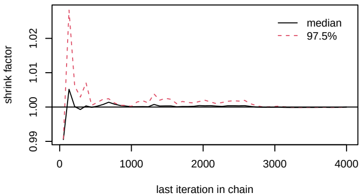
gamma[6,1]
