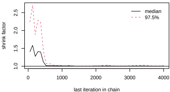
alpha1[4]
