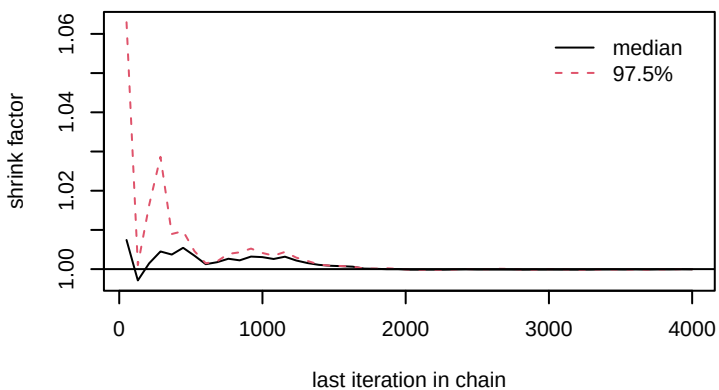
gamma[3,4]
