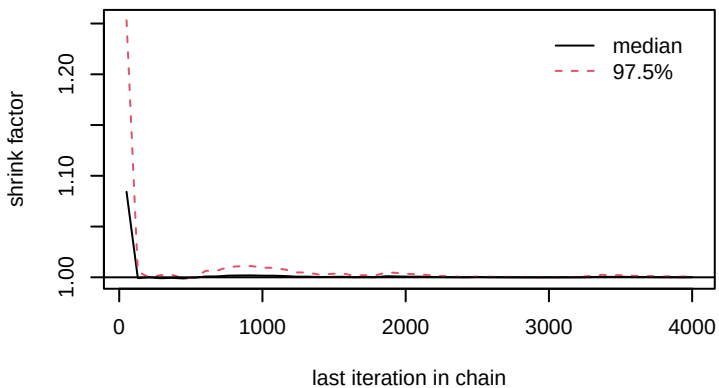
lambda0[3]
