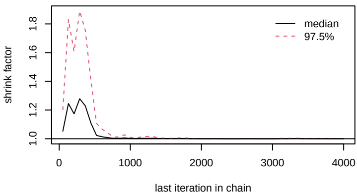
alpha1[1]
