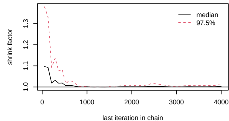
alpha1[6]
