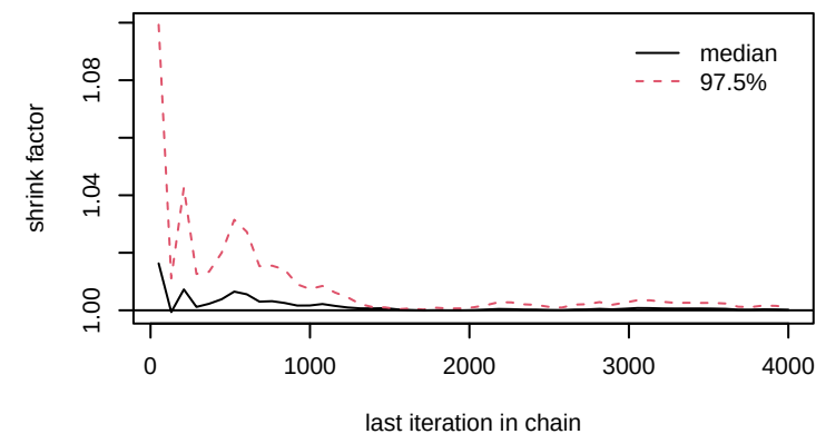
gamma[8,4]
