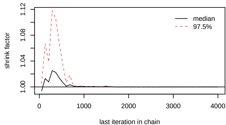
gamma[1,1]
