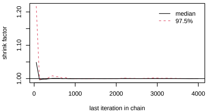
gamma[9,5]
