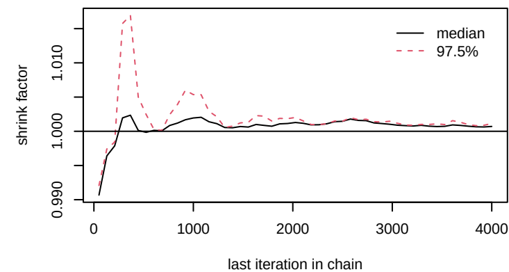
gamma[8,5]
