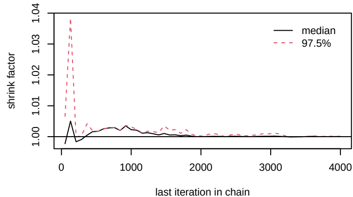
gamma[4,4]
