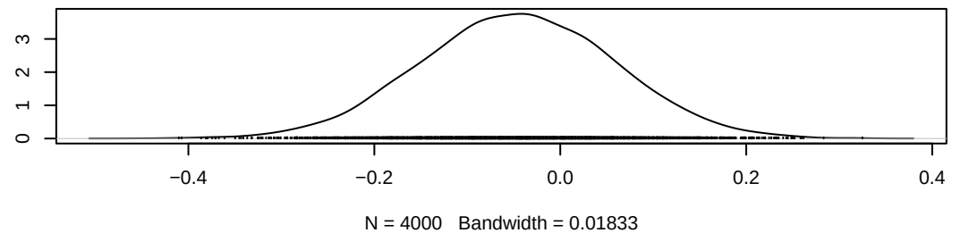
Density of alpha0[6]
