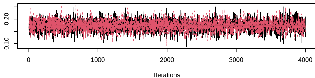
Trace of gamma[5,8]
