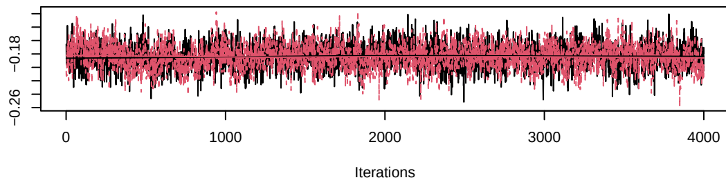
Trace of alpha0[5]
