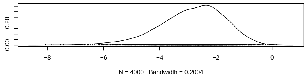
Density of gamma[7,2]
