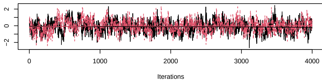
Trace of alpha1[8]
