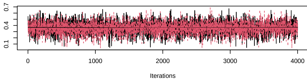
Trace of gamma[5,5]
