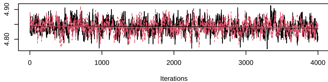
Trace of beta0_y
