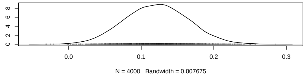
Density of gamma[5,3]
