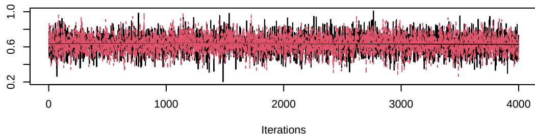
Trace of gamma[2,1]
