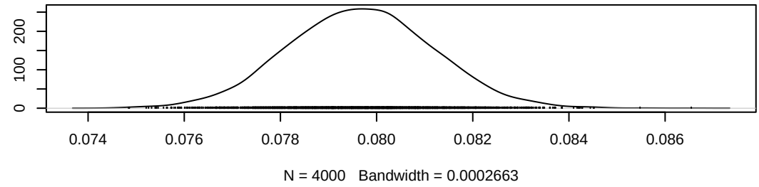
Density of lambda0[1]
