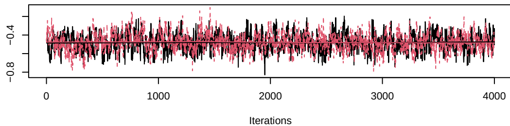
Trace of beta_long[5]
