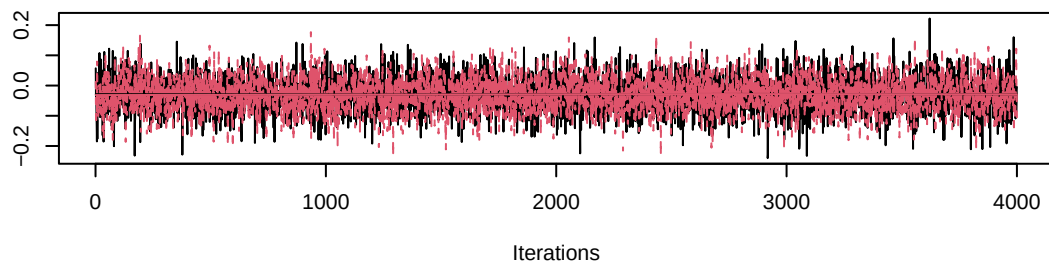
Trace of gamma[8,3]
