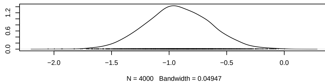
Density of alpha1[1]
