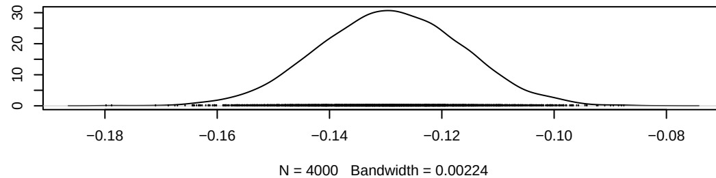
Density of alpha0[1]
