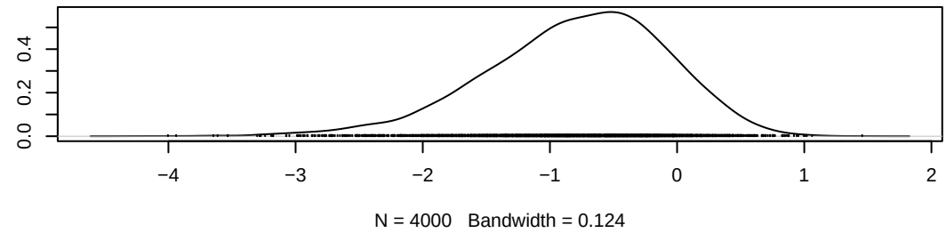
Density of gamma[3,7]
