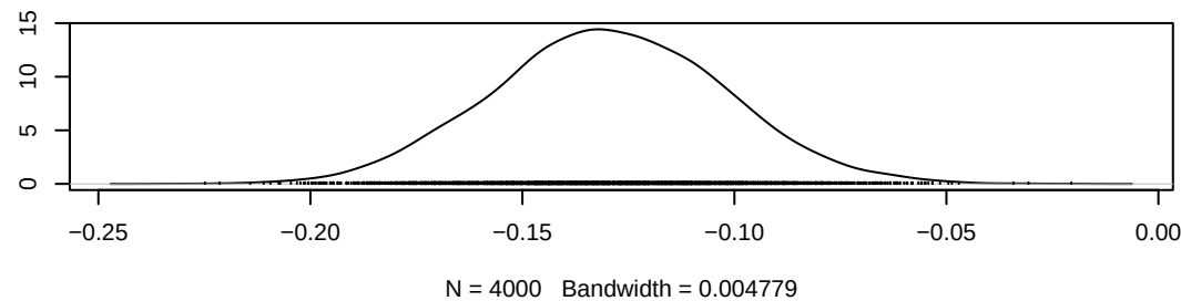
Density of gamma[8,8]
