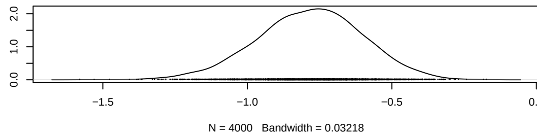
Density of gamma[4,5]
