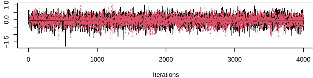
Trace of gamma[9,4]
