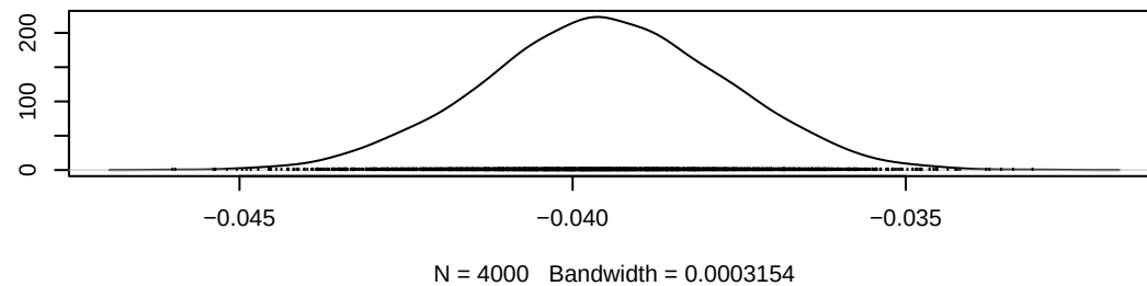
Density of beta_time_y
