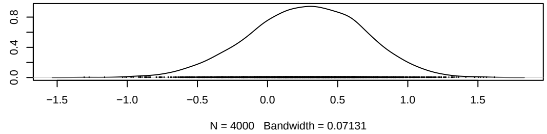
Density of gamma[3,3]
