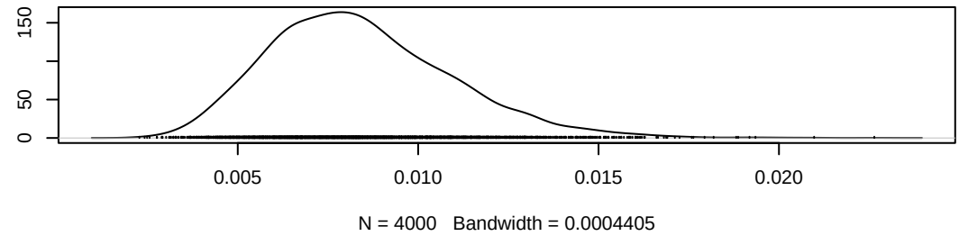
Density of lambda0[7]
