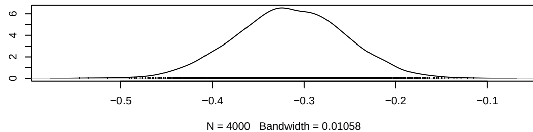
Density of beta_long[4]
