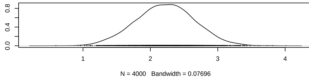
Density of alpha1[4]
