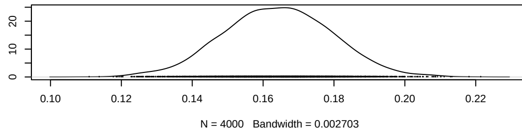
Density of gamma[1,8]
