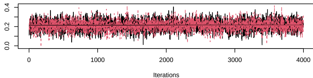
Trace of gamma[5,2]
