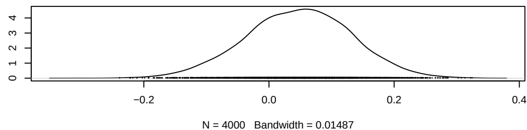
Density of gamma[5,6]
