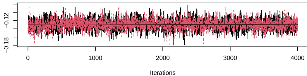
Trace of alpha0[1]
