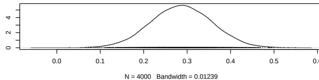
Density of gamma[5,4]
