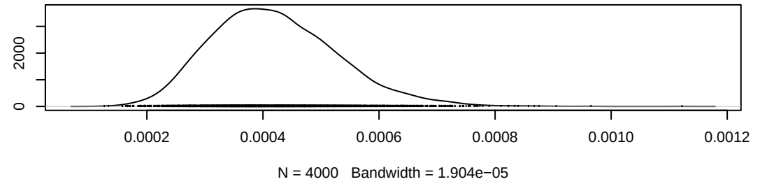
Density of lambda0[3]
