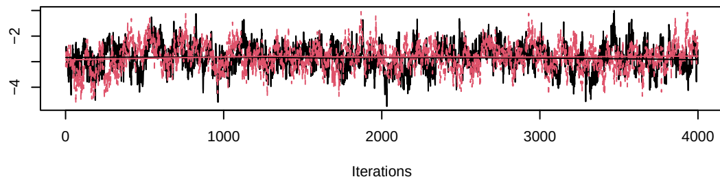
Trace of alpha1[5]
