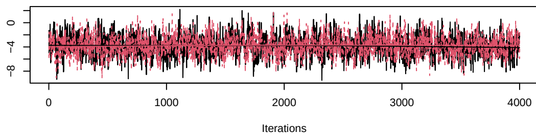
Trace of alpha1[2]
