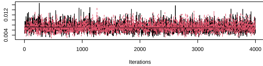
Trace of lambda0[9]
