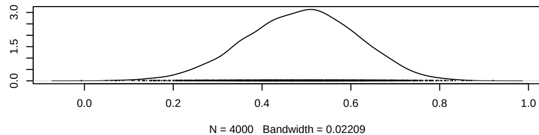
Density of gamma[1,5]
