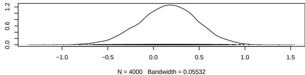
Density of gamma[6,2]
