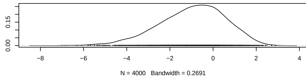
Density of gamma[3,5]
