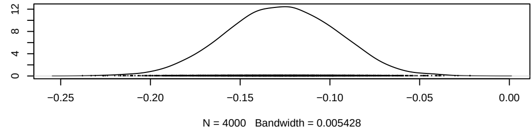
Density of gamma[8,1]
