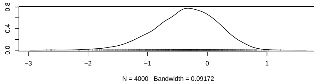
Density of gamma[6,4]
