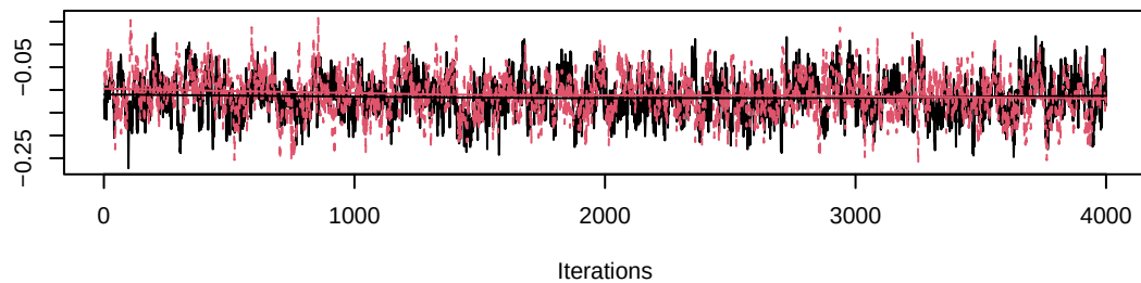
Trace of beta_long[2]
