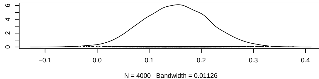
Density of beta_long[6]
