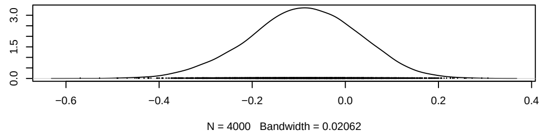
Density of gamma[8,6]
