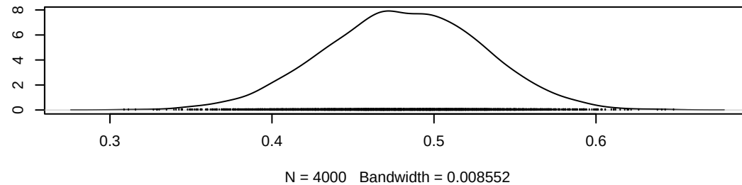
Density of gamma[1,2]
