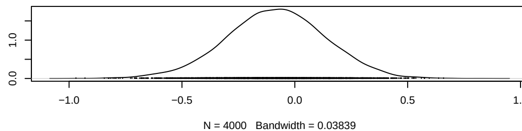
Density of gamma[9,3]
