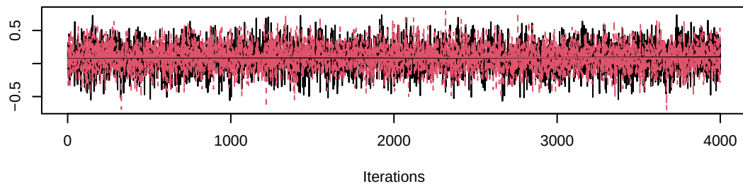
Trace of gamma[2,3]
