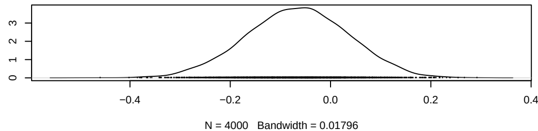
Density of gamma[9,8]
