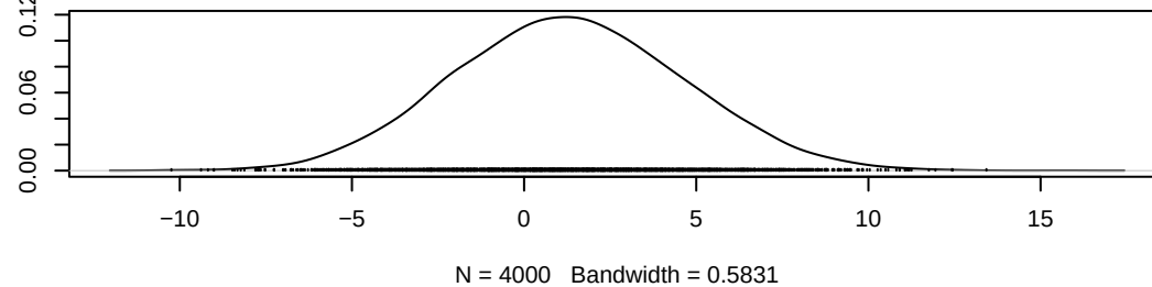
Density of alpha1[7]
