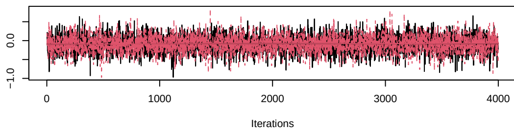
Trace of gamma[9,3]
