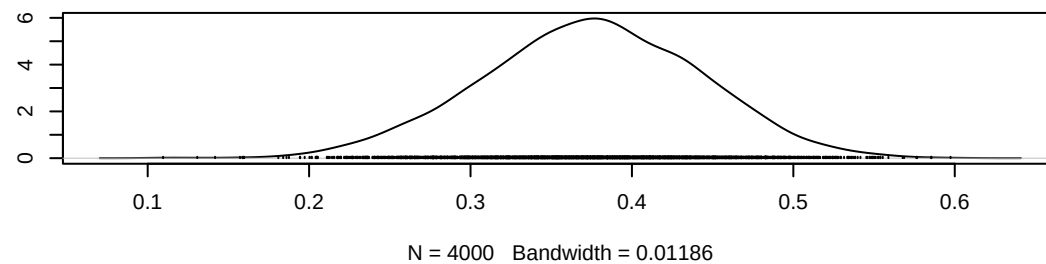
Density of gamma[1,4]
