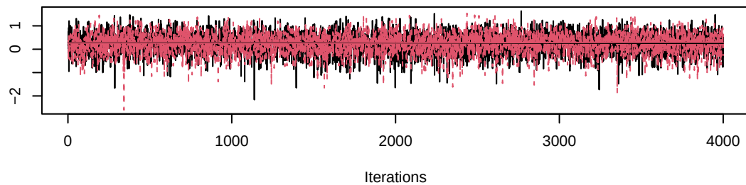
Trace of gamma[2,4]
