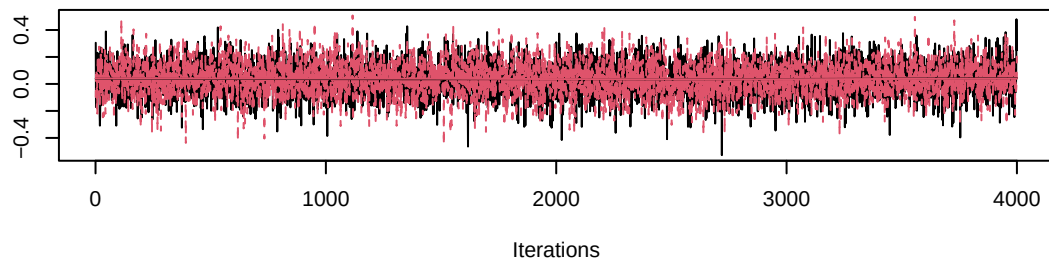
Trace of gamma[6,8]
