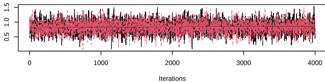
Trace of gamma[3,1]
