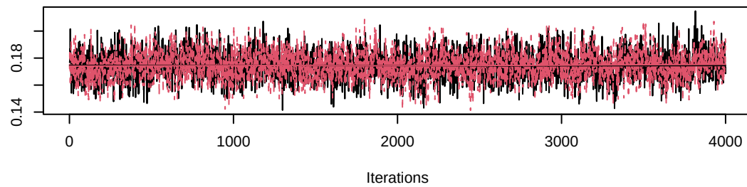
Trace of lambda0[8]
