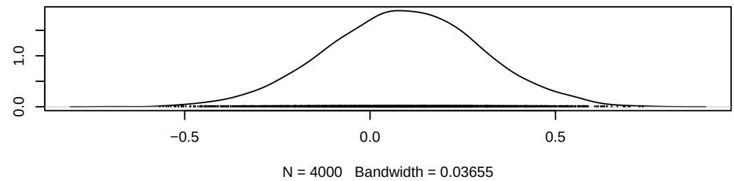
Density of gamma[2,3]
