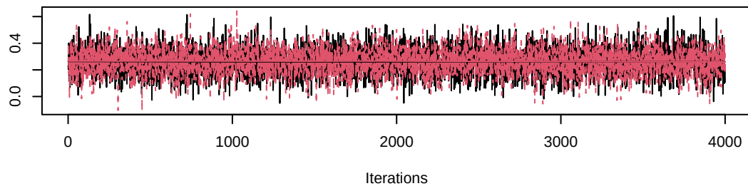
Trace of gamma[2,8]
