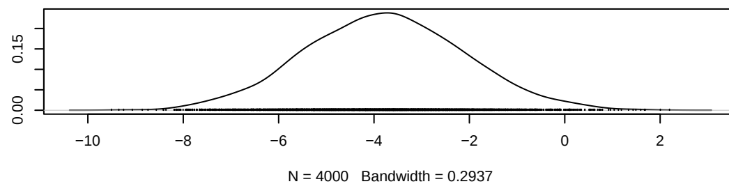
Density of alpha1[2]
