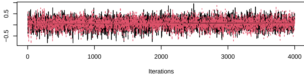
Trace of gamma[9,2]
