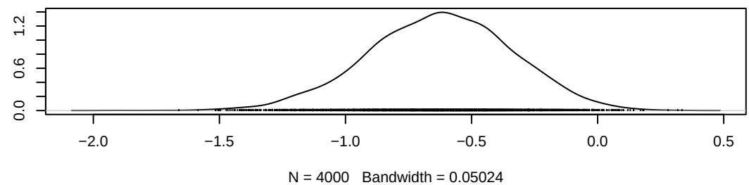
Density of gamma[6,7]
