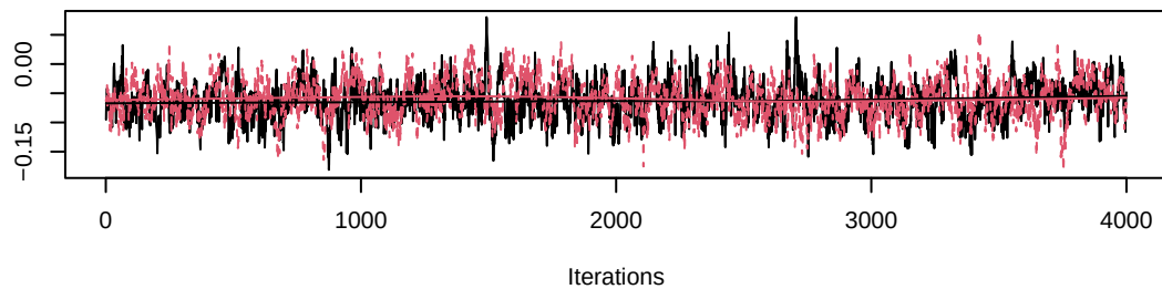
Trace of beta_long[7]
