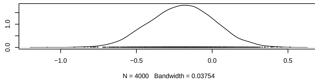
Density of gamma[3,8]
