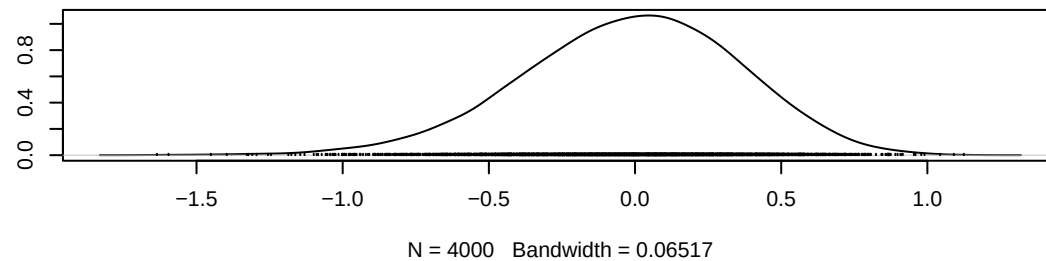
Density of gamma[2,2]
