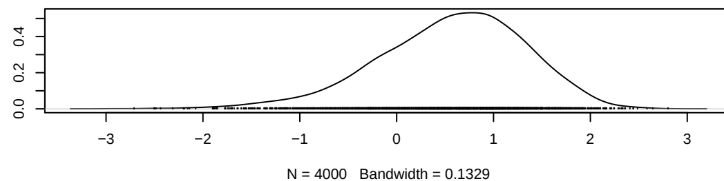
Density of gamma[3,4]
