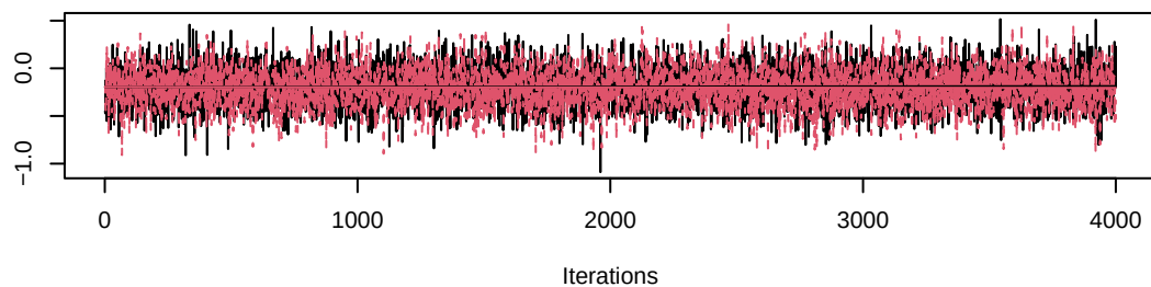
Trace of gamma[3,8]
