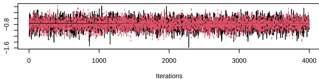
Trace of gamma[4,5]
