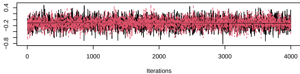
Trace of alpha0[3]
