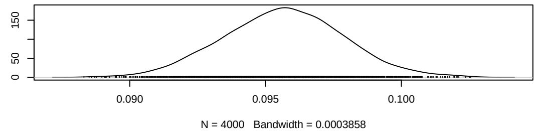
Density of sigma_b1
