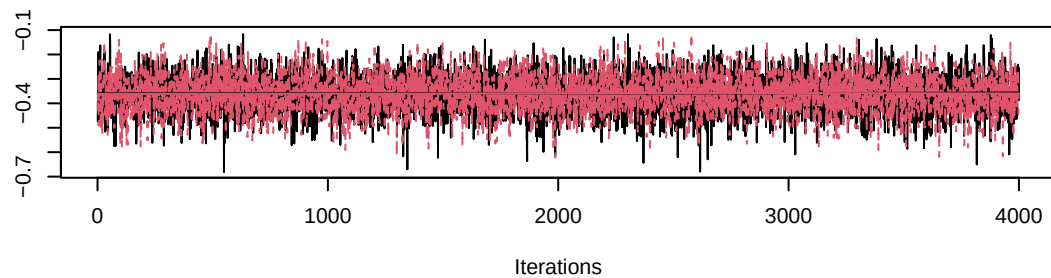
Trace of gamma[4,6]
