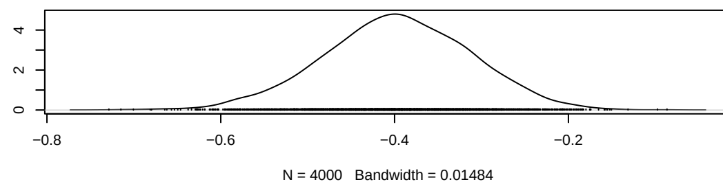
Density of gamma[4,4]
