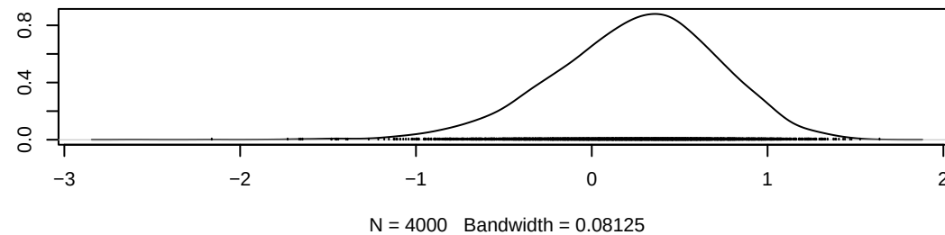
Density of gamma[2,4]
