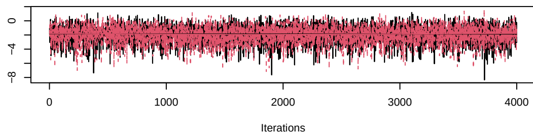
Trace of gamma[7,6]
