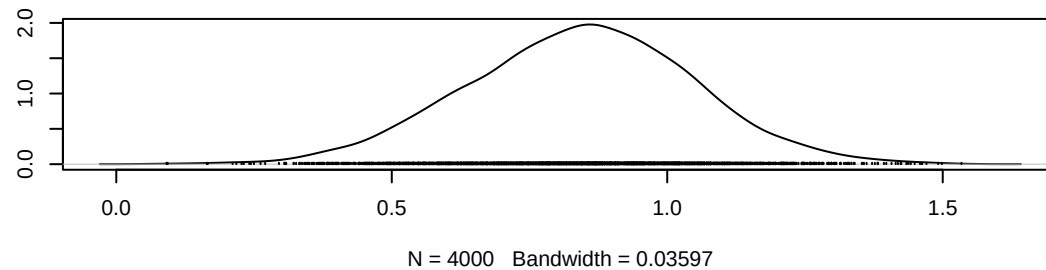
Density of gamma[3,1]
