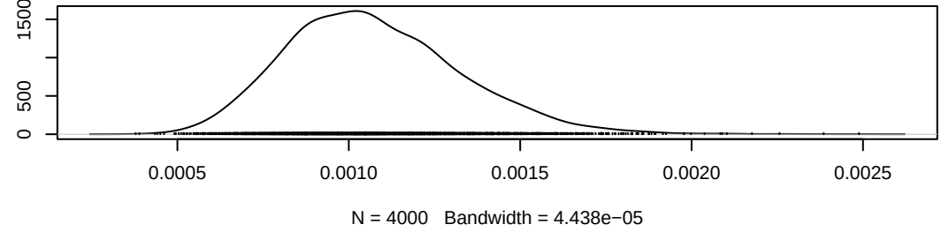
Density of lambda0[6]
