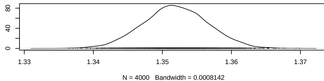
Density of sigma_y
