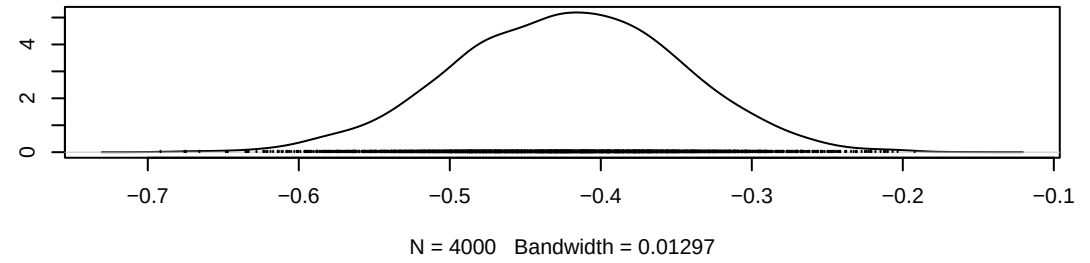
Density of gamma[8,2]
