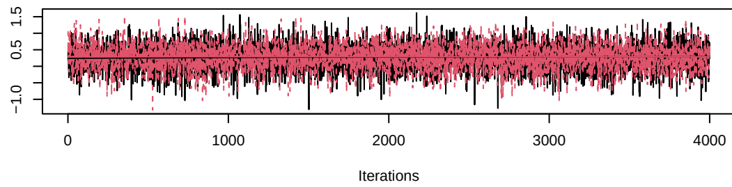
Trace of gamma[3,3]
