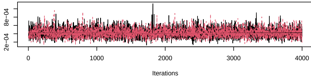
Trace of lambda0[3]
