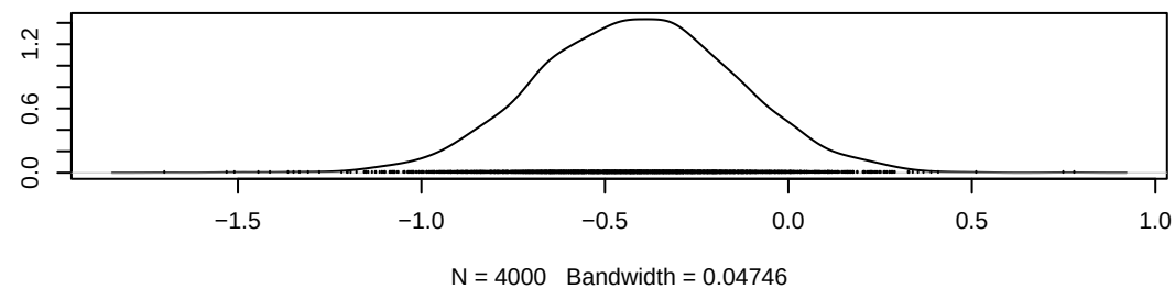
Density of gamma[6,3]
