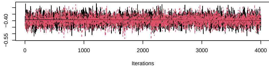
Trace of gamma[4,3]
