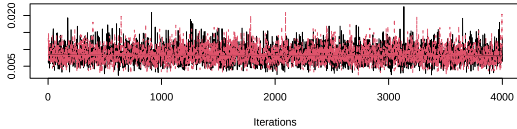
Trace of lambda0[7]
