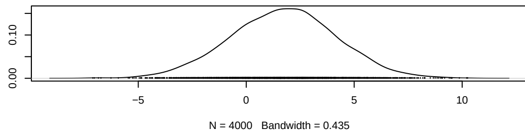
Density of alpha1[9]
