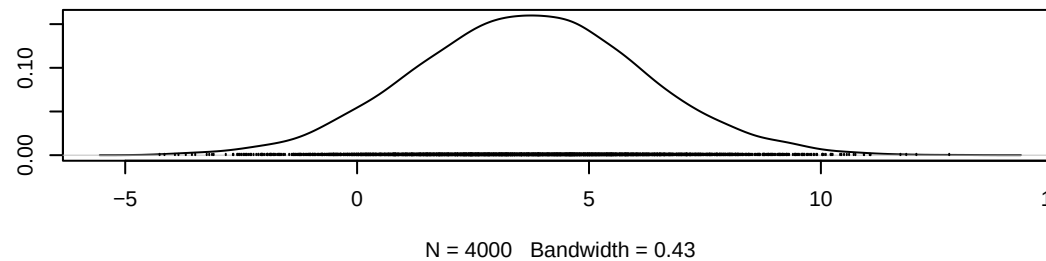
Density of alpha1[6]
