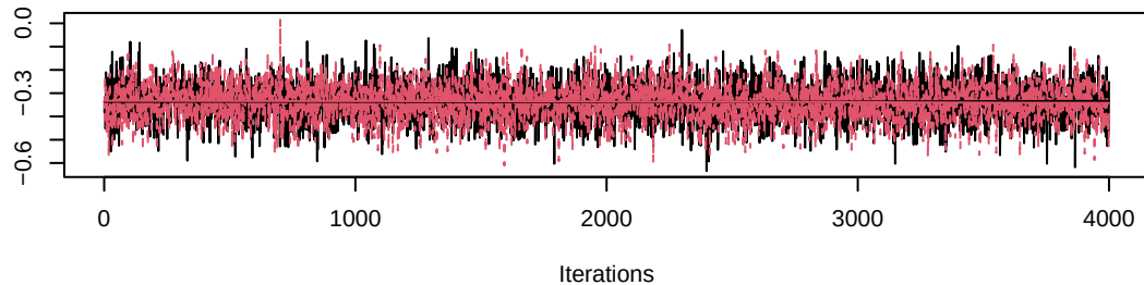
Trace of alpha0[2]
