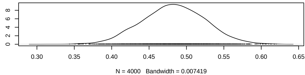
Density of gamma[5,7]
