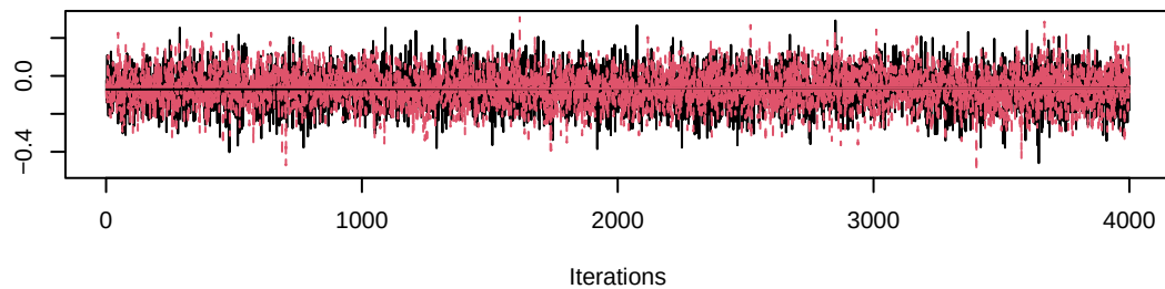
Trace of gamma[9,8]
