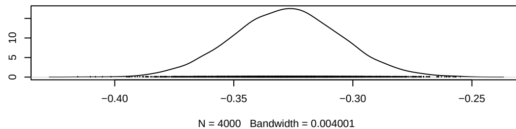
Density of gamma[4,1]
