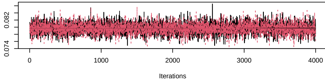
Trace of lambda0[1]
