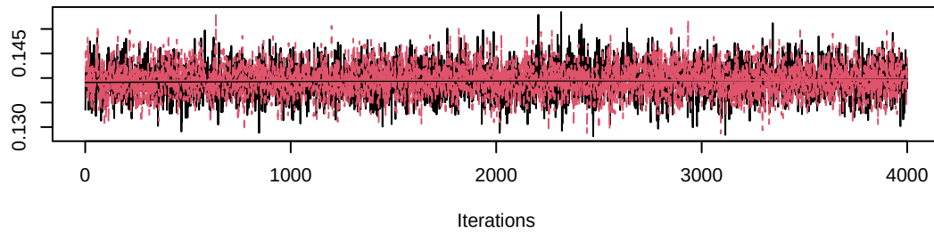
Trace of lambda0[4]
