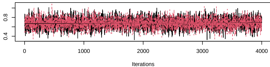
Trace of gamma[9,1]
