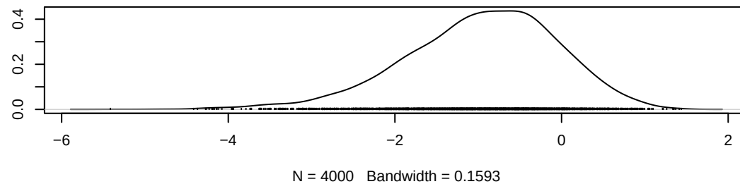
Density of gamma[7,4]
