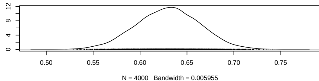
Density of gamma[1,7]
