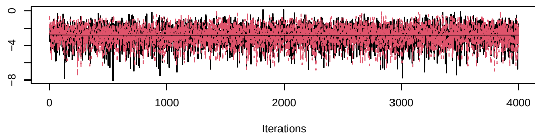
Trace of gamma[7,2]
