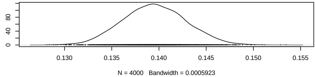
Density of lambda0[4]
