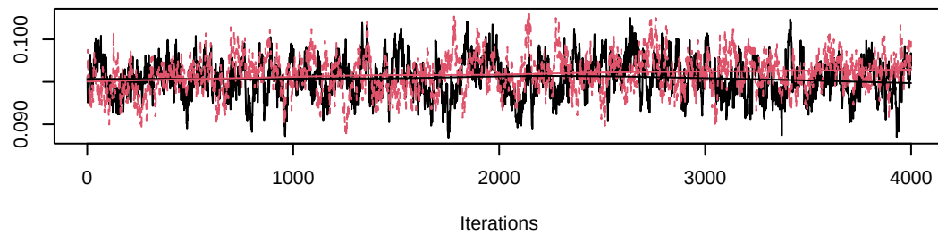
Trace of sigma_b1
