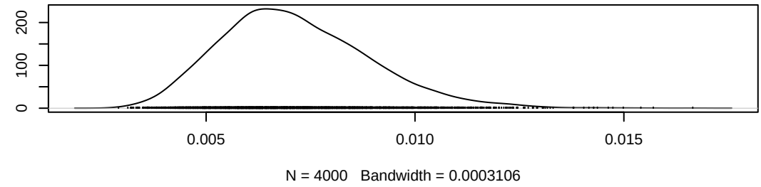
Density of lambda0[9]
