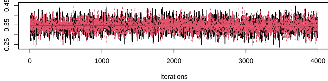
Trace of gamma[1,3]
