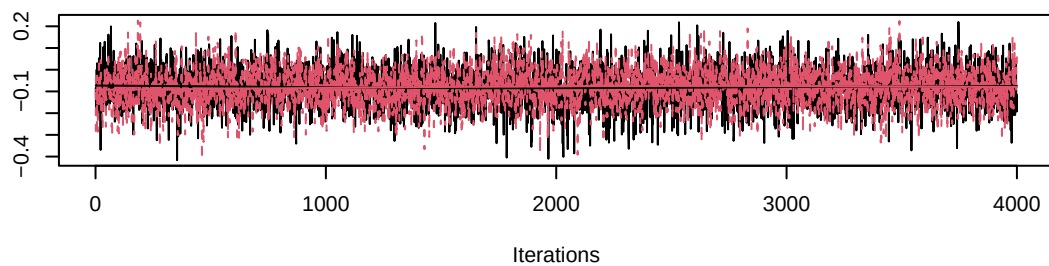
Trace of alpha0[9]
