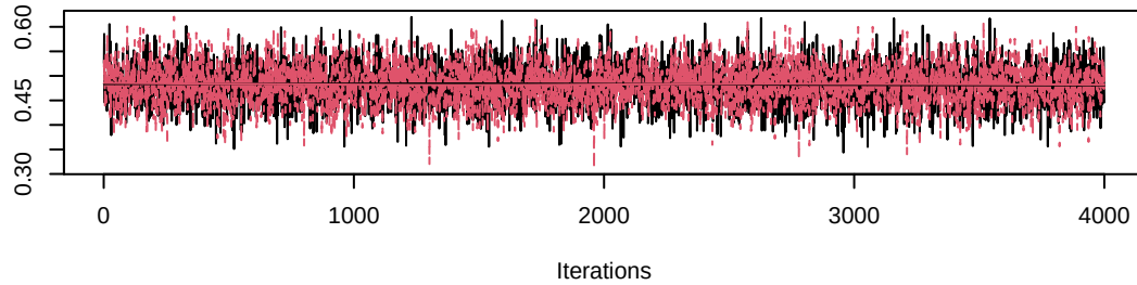
Trace of gamma[5,7]
