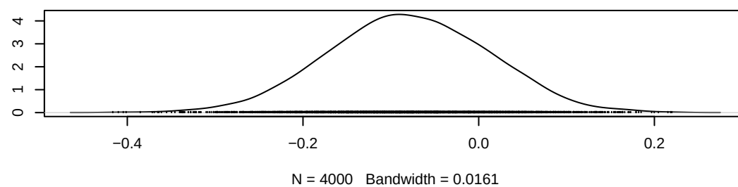
Density of alpha0[9]
