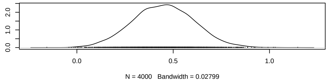
Density of alpha0[7]
