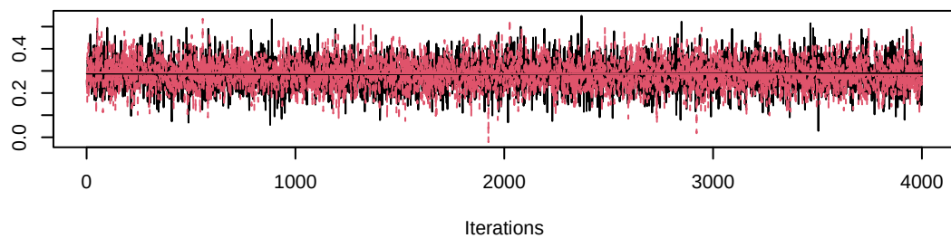
Trace of gamma[5,4]
