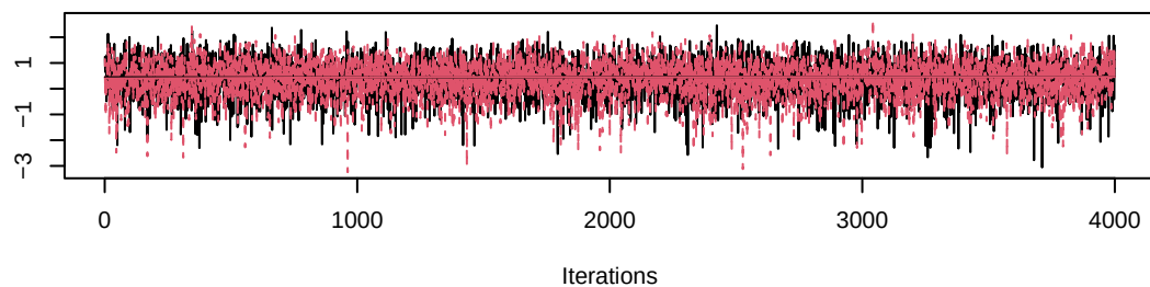
Trace of gamma[2,5]
