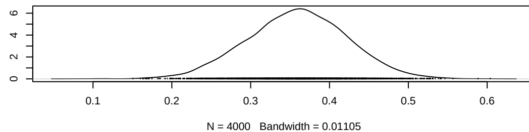
Density of gamma[1,6]
