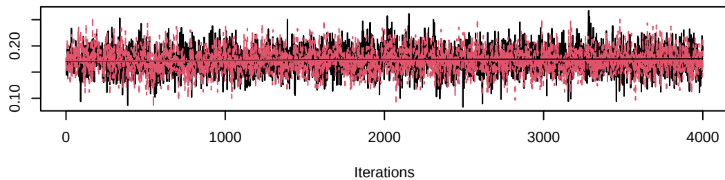
Trace of alpha0[8]
