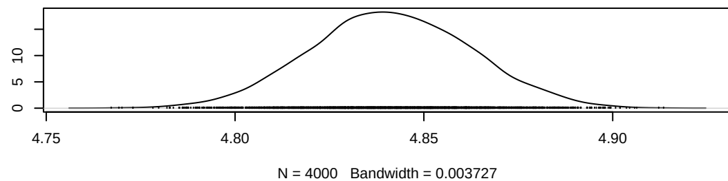
Density of beta0_y
