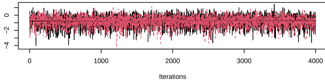
Trace of gamma[3,7]
