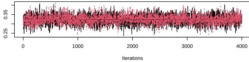
Trace of gamma[5,1]
