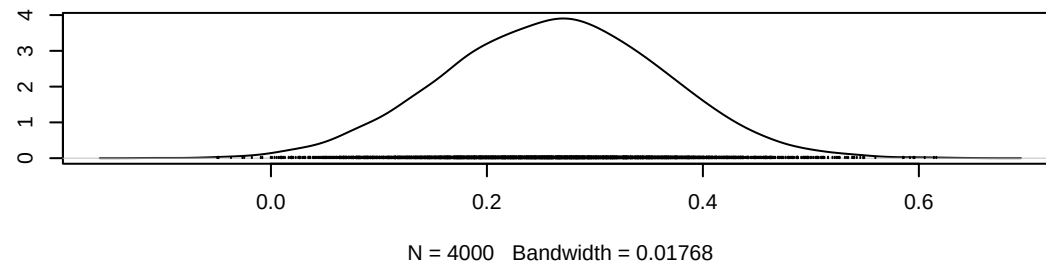
Density of gamma[2,8]
