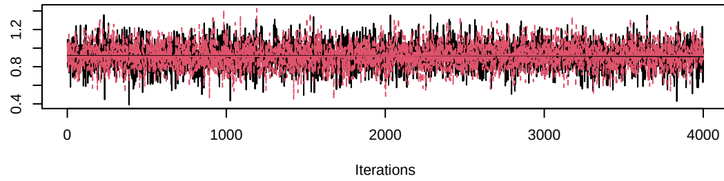
Trace of gamma[6,1]
