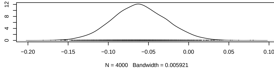
Density of beta_long[7]
