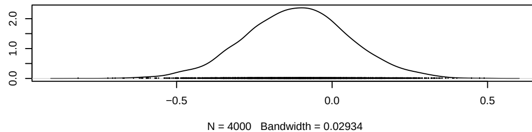
Density of alpha0[3]
