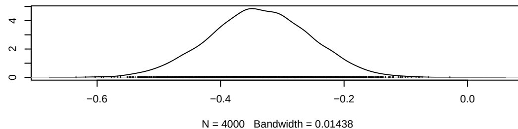
Density of alpha0[2]
