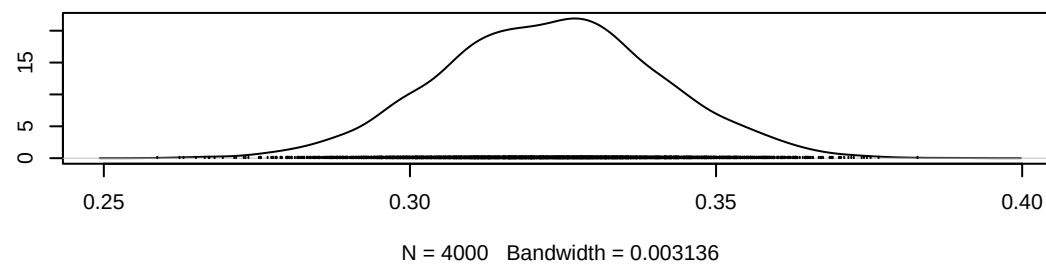
Density of gamma[1,1]
