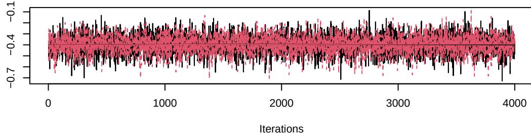
Trace of gamma[4,4]
