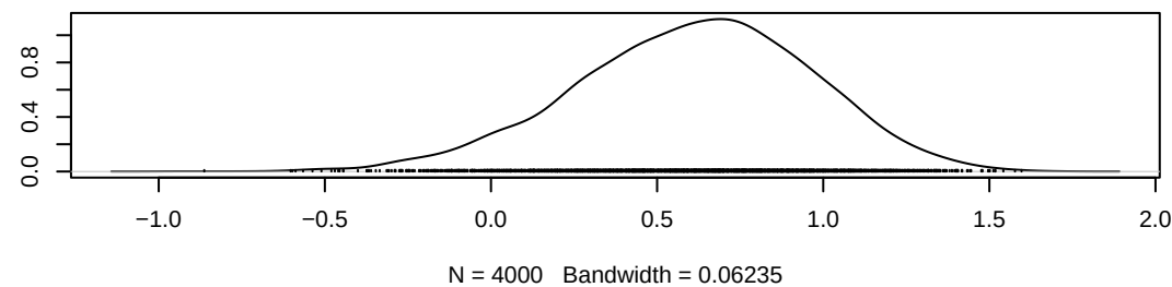
Density of gamma[2,6]
