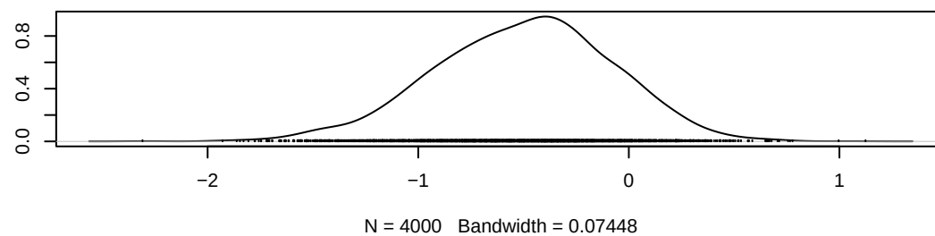
Density of gamma[7,3]
