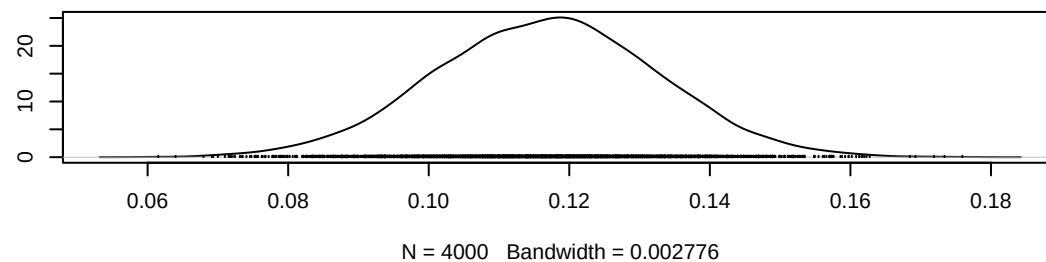
Density of alpha0[4]
