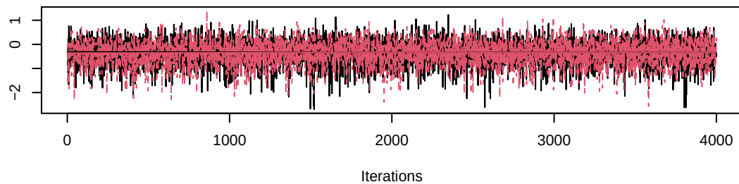
Trace of gamma[6,4]
