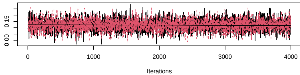
Trace of gamma[5,3]
