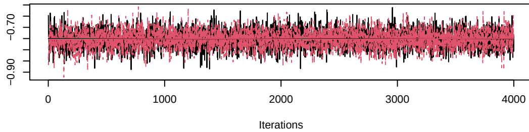
Trace of gamma[4,7]
