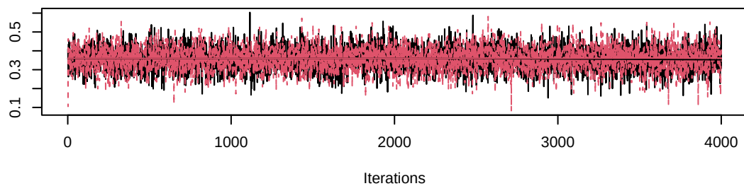
Trace of gamma[1,6]
