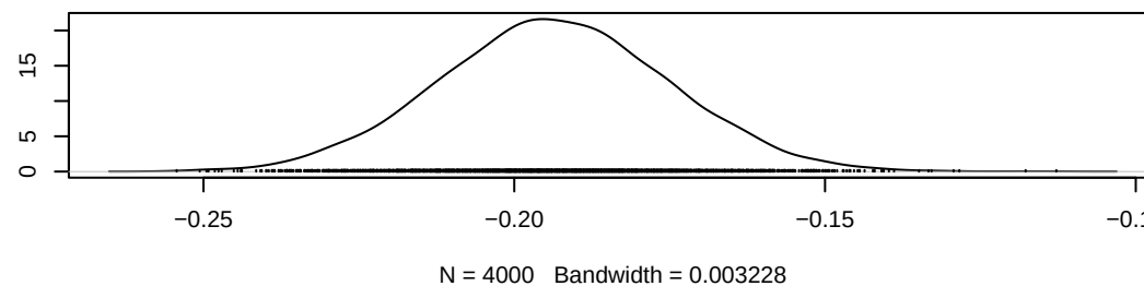
Density of gamma[4,8]
