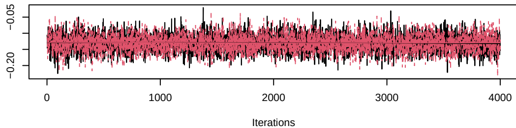
Trace of gamma[8,8]
