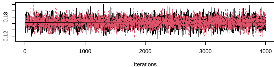
Trace of gamma[1,8]
