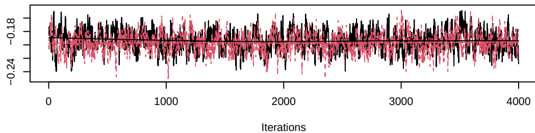
Trace of beta_long[8]
