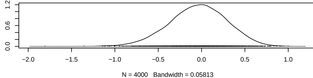
Density of gamma[9,4]
