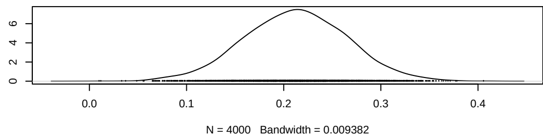
Density of gamma[5,2]
