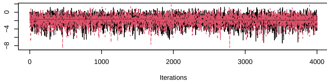
Trace of gamma[7,5]
