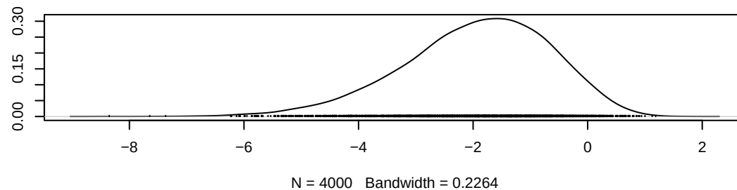
Density of gamma[7,6]
