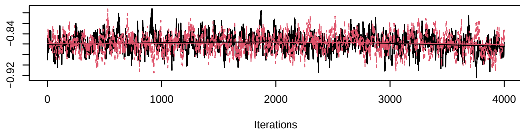
Trace of beta_long[1]
