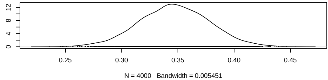
Density of gamma[1,3]
