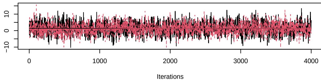
Trace of alpha1[7]
