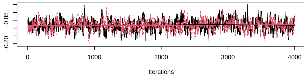
Trace of beta_long[3]
