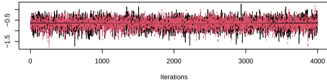
Trace of gamma[7,1]
