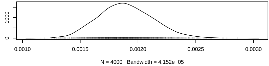
Density of lambda0[2]
