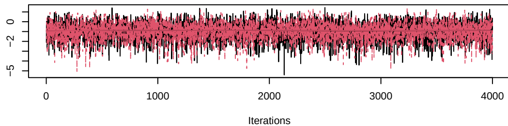
Trace of gamma[7,4]
