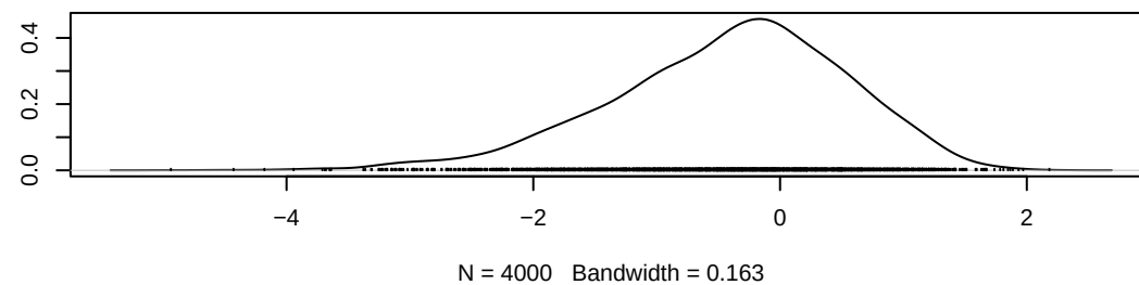
Density of gamma[3,6]
