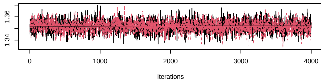
Trace of sigma_y
