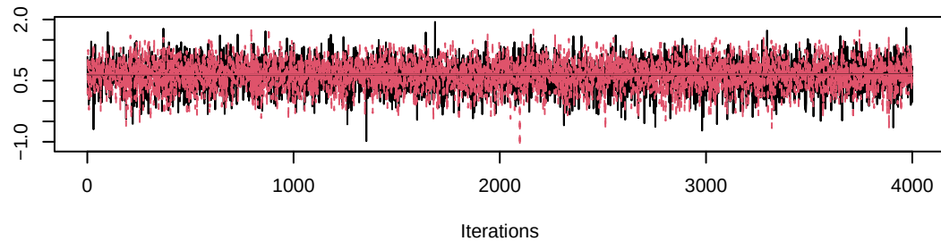
Trace of gamma[6,6]
