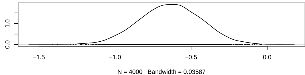
Density of gamma[7,8]
