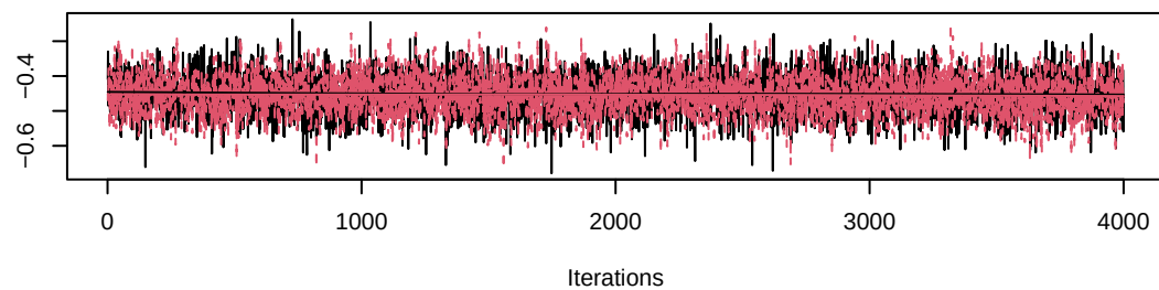
Trace of gamma[4,2]
