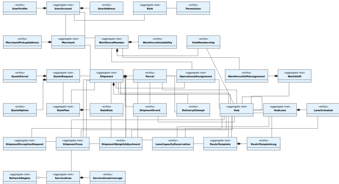
PAVEX Domain Model - entities
