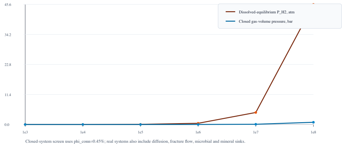
Closed-system H2 accumulation screen from host-rock radiolysis
