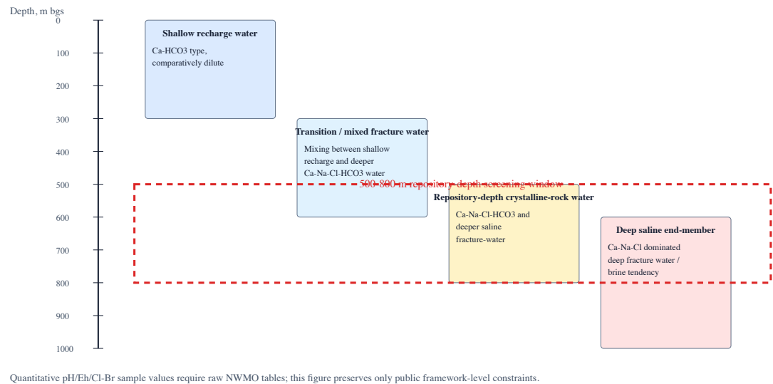
Revell groundwater chemistry depth framework
