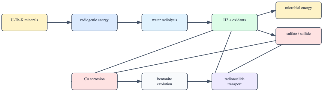
Safety-relevant reaction pathway map
