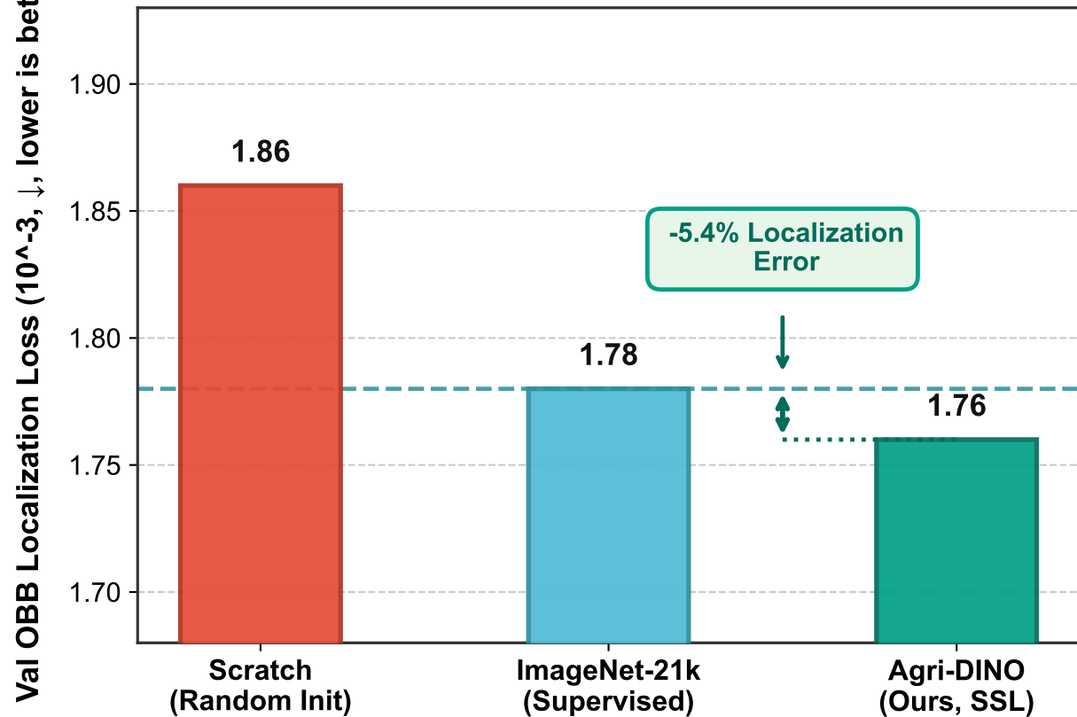
(b) PlantSeg OBB Disease Lesion Localization Loss
