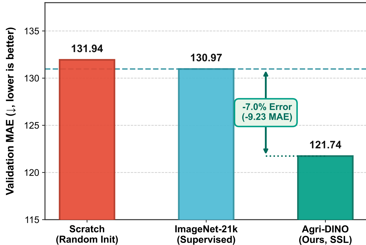
(a) Dense Spatial Corn Kernel Counting MAE
