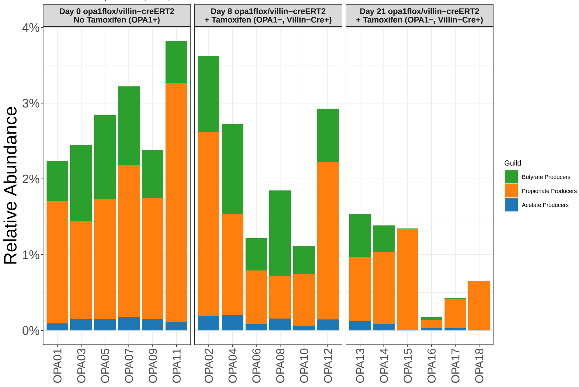
Figure 5D — SCFA producer guild contributions per sample
