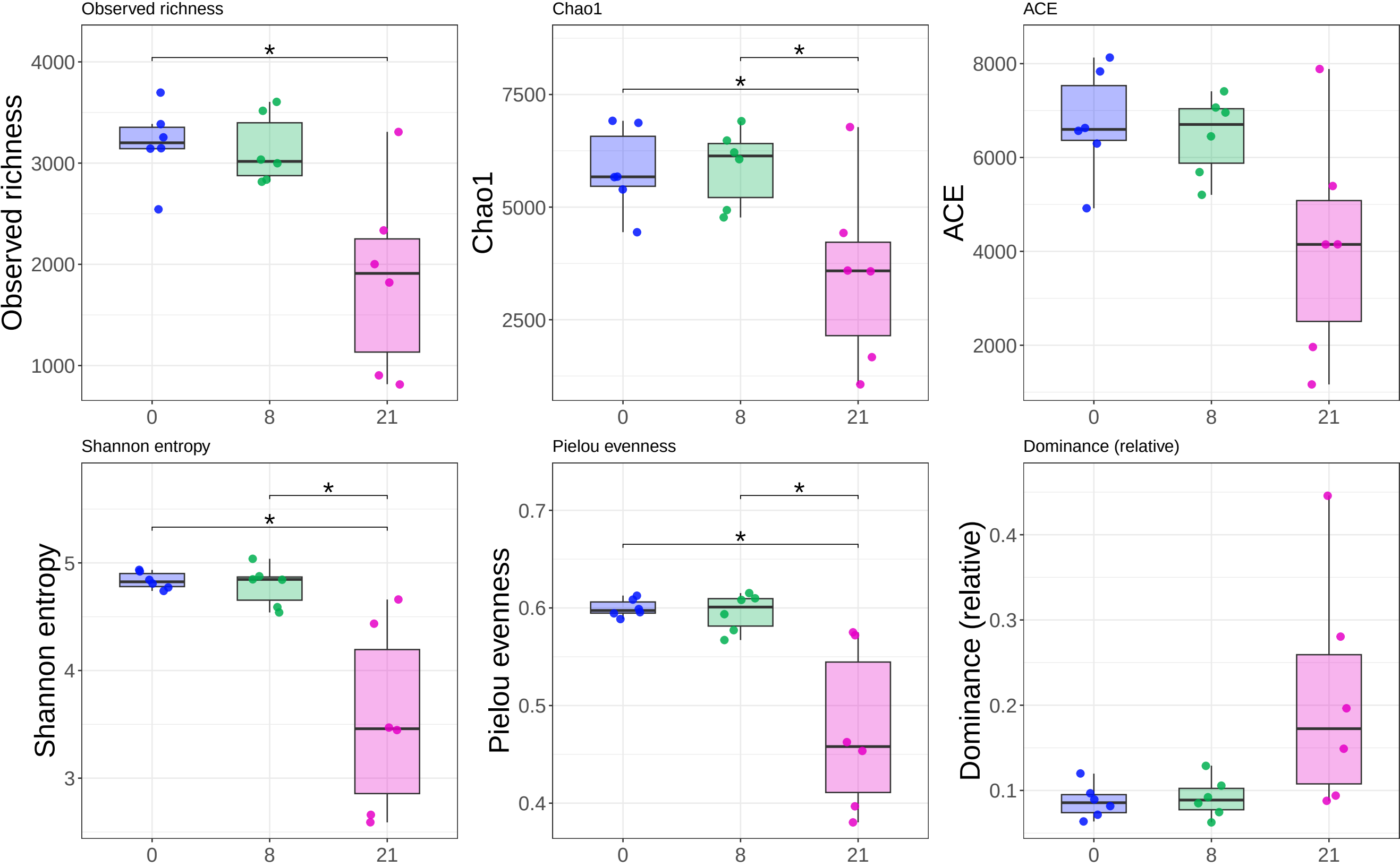
Figure 4A — Alpha diversity (S2: OPA1 KO longitudinal)
