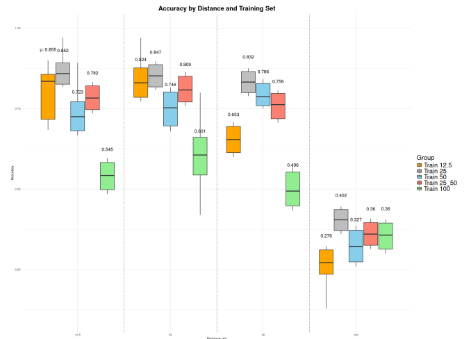
Figure 16: Accuracy Boxplots obtained from test set after training on different distances
