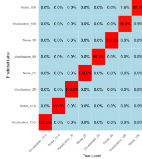
Figure 14: Confusion matrix of the random forest classifier trained and tested on DataVocNoise (in % of correct classification on the test set).
