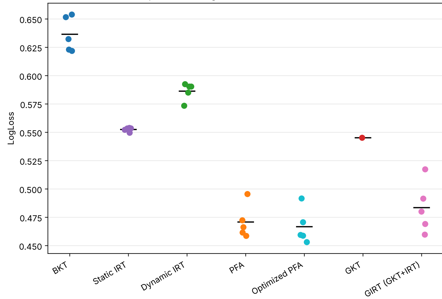
Dispersion of LogLoss across folds (— = mean)
