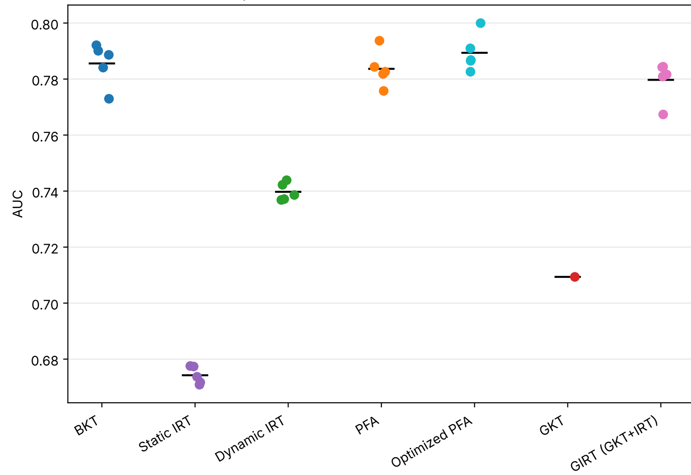
Dispersion of AUC across folds (— = mean)
