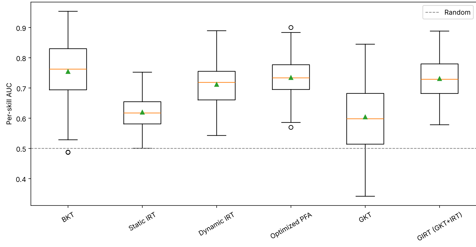
Per-skill AUC distribution
