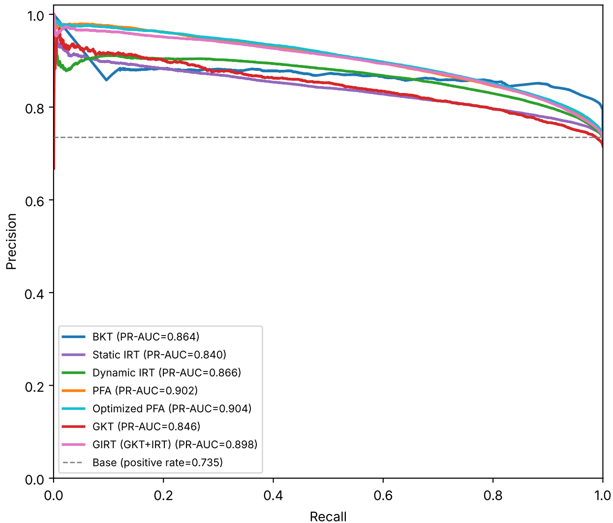
Precision-Recall curves — all models
