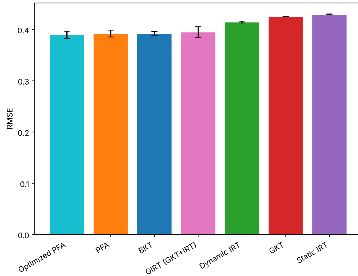
RMSE per model (↓ better) — mean ± std over 5 folds
