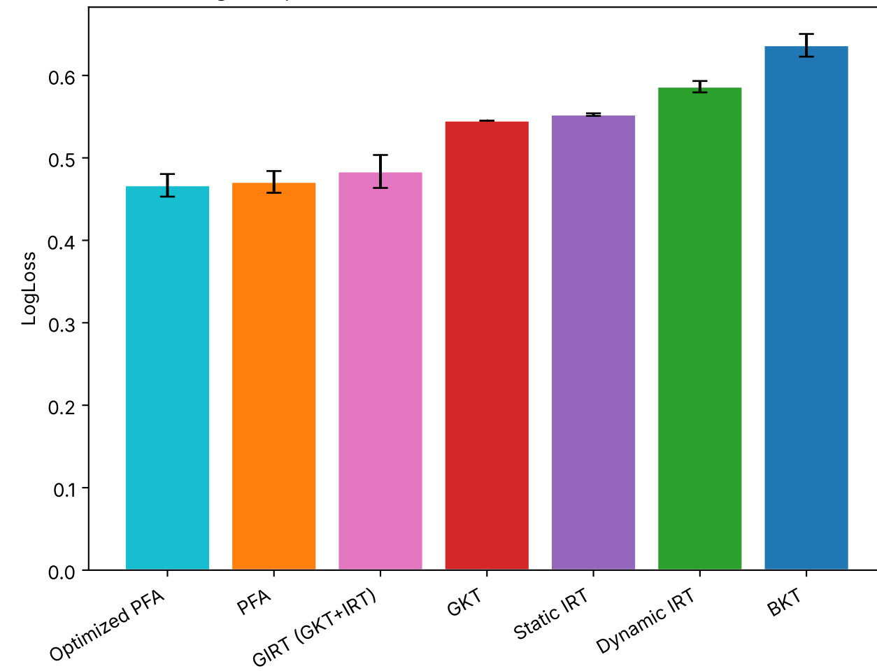
LogLoss per model (↓ better) — mean ± std over 5 folds
