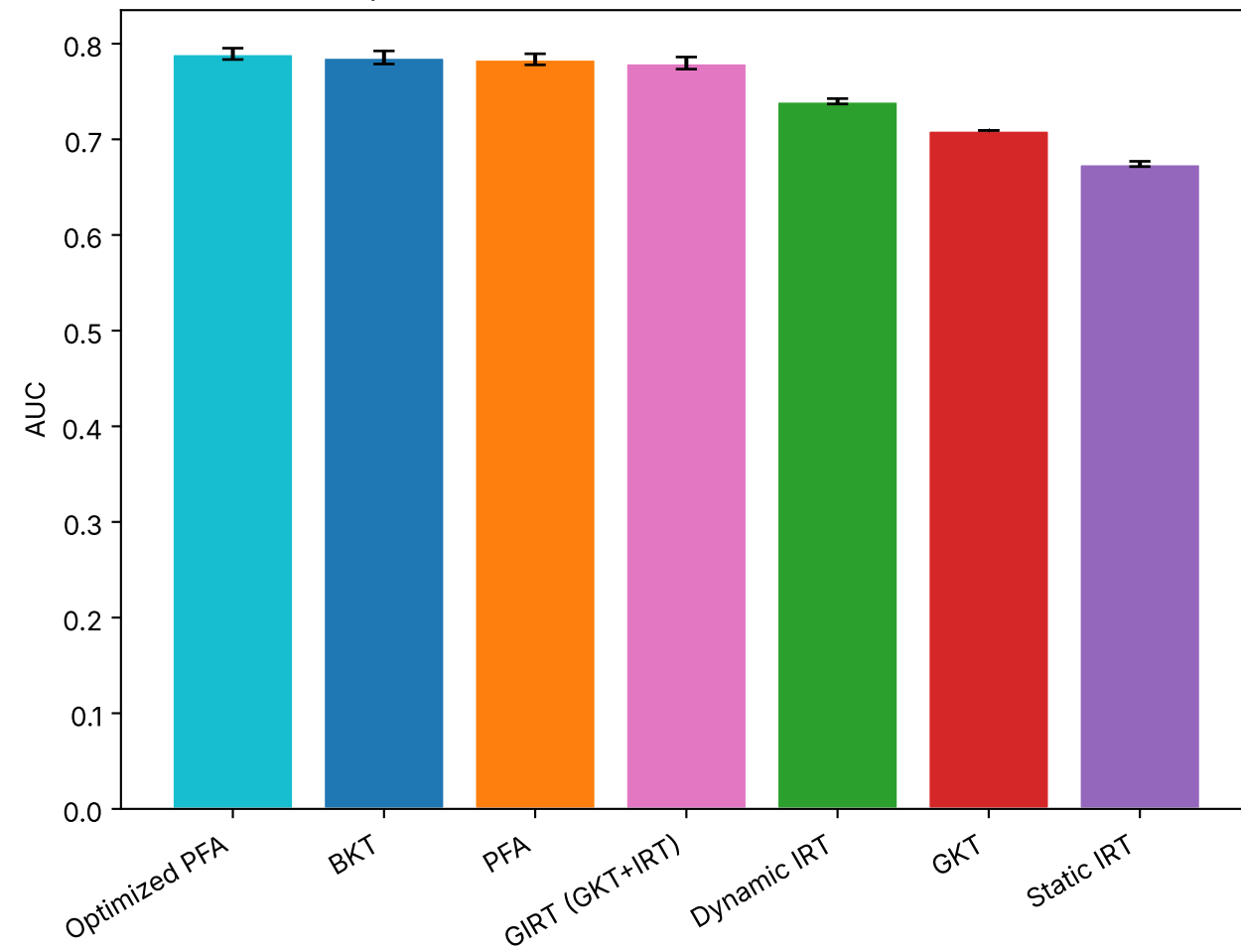
AUC per model (↑ better) — mean ± std over 5 folds
