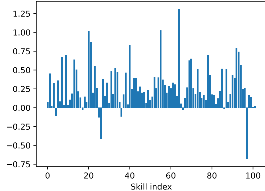
alpha_k - ELO learning rate per skill (high = ability updates fast)
