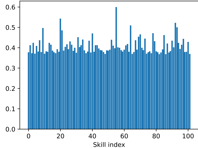
\sigma_k - variability of progress per skill (high = inconsistent learning)
