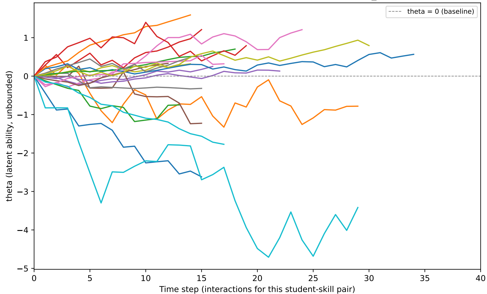
Theta trajectories (subset of students/skills) Rising = learning, Falling = struggling, Drift = \mu_k
