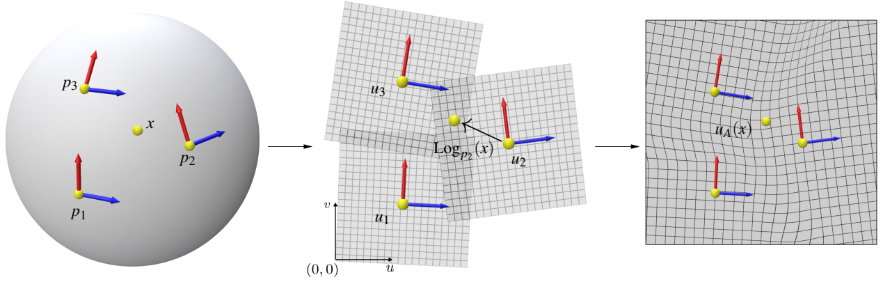
Figure 9: To combine multiple uv-fields, we wish to take weighted averages of coordinates at a point x , coming from adjacent seeds (left). Since each Log map \text{Log}_{p_i} is expressed in its own referential, we first assign each seed p_i an offset coordinate u_i \in \mathbb{R}^2 in a common uv-space (middle). In this common coordinate system, we can blend the coordinates at the interfaces between the seeds using compact support interpolation (right).
