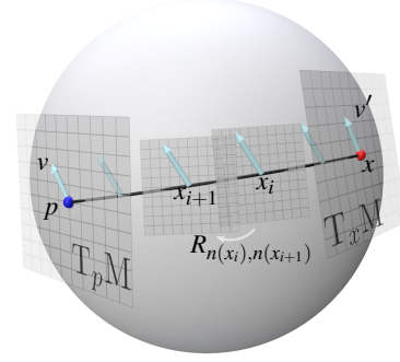
Figure 6: We can discretize parallel transport along the curve built by Alg. 1. We store the product of each rotation matrix R_{n(x_i), n(x_{i+1})} into one rotation matrix R_{p \rightarrow x} . A vector v \in T_pM is then transported to v' \in T_xM by v' = R_{p \rightarrow x}v .
