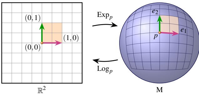
Figure 4: With a selected orthonormal frame e_1, e_2 \in T_p M , the exponential map \text{Exp}_p maps a flat plane to the surface, while the log map \text{Log}_p provides each nearby point x with 2D coordinates.
