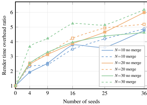
Figure 15: Plot of the render time (shown as ratio to render time without seeds) with increasing number of seeds, with and without merging. The seeds are placed uniformly on a flat geometry and rendered from a fixed camera. We tested different numbers of geodesic tracing iterations N = 10, 20, 30 and with or without merging. Timings were captured on a MacBook Pro M1 Max.
