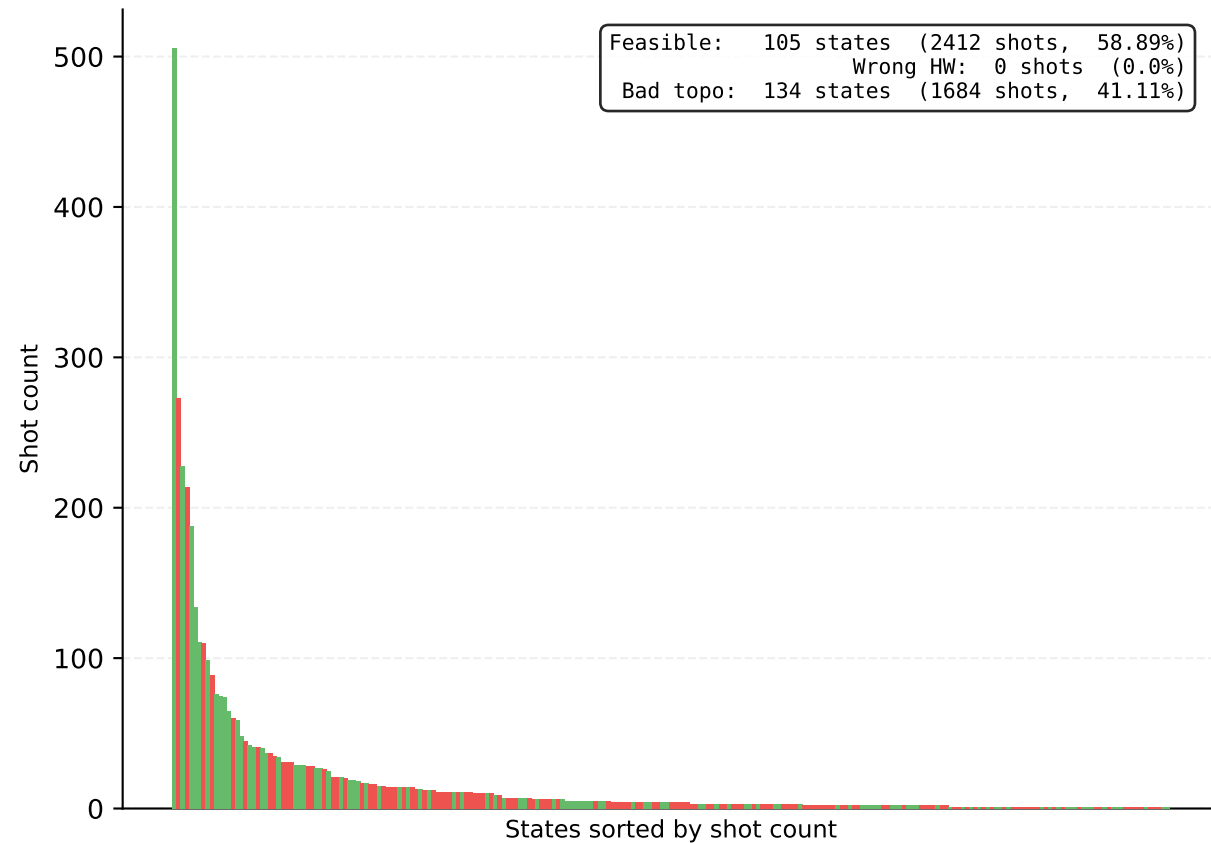
[Exact Sim] NN-2 AOA | 12-bus | 239 unique / 4096 shots
