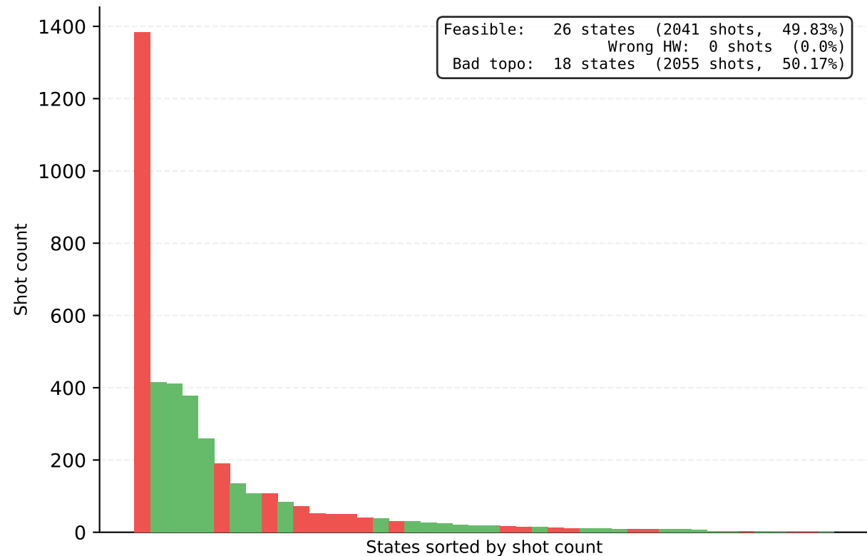
[Exact Sim] NN-2 AOA | 44 unique / 4096 shots
