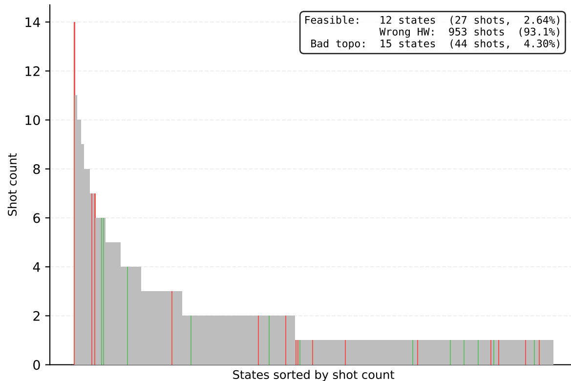
[Noisy Sim] NN-2 AOA | 484 unique / 1024 shots
