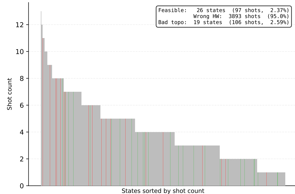
[QPU ibm_fez] NN-2 AOA | 986 unique / 4096 shots
