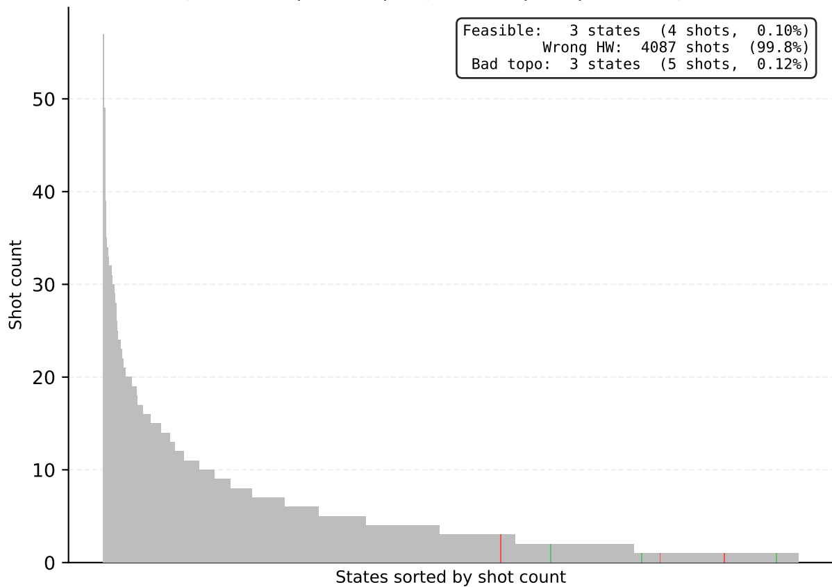
NN-2 QAOA (qamomile) | 9-bus | depth=13 | 1L | 137 unique / 4096 shots
