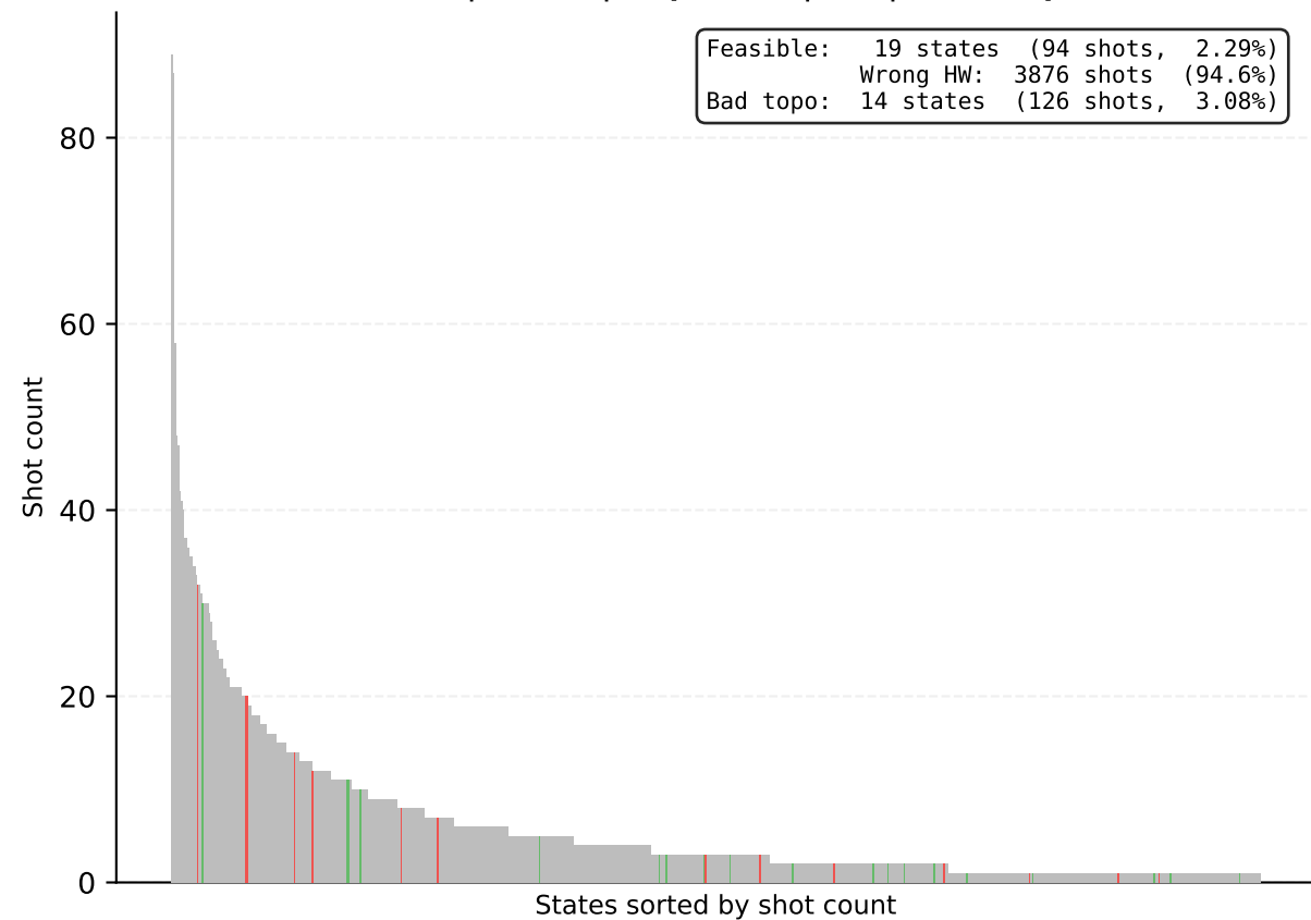
NN-2 QAOA (native) | 9-bus | depth=28 | 1L | 663 unique / 4096 shots
