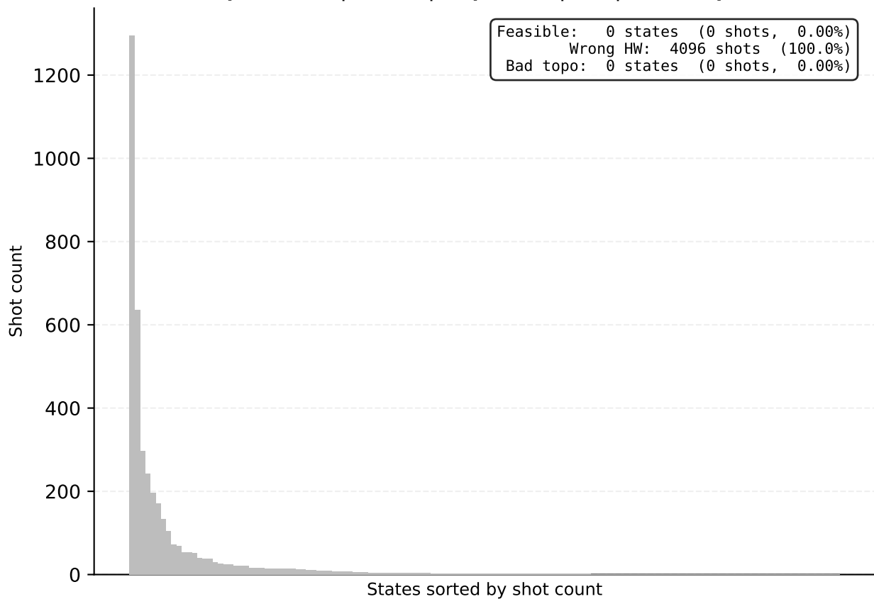
NN-2 QAOA (qamomile) | 9-bus | depth=13 | 1L | 137 unique / 4096 shots
