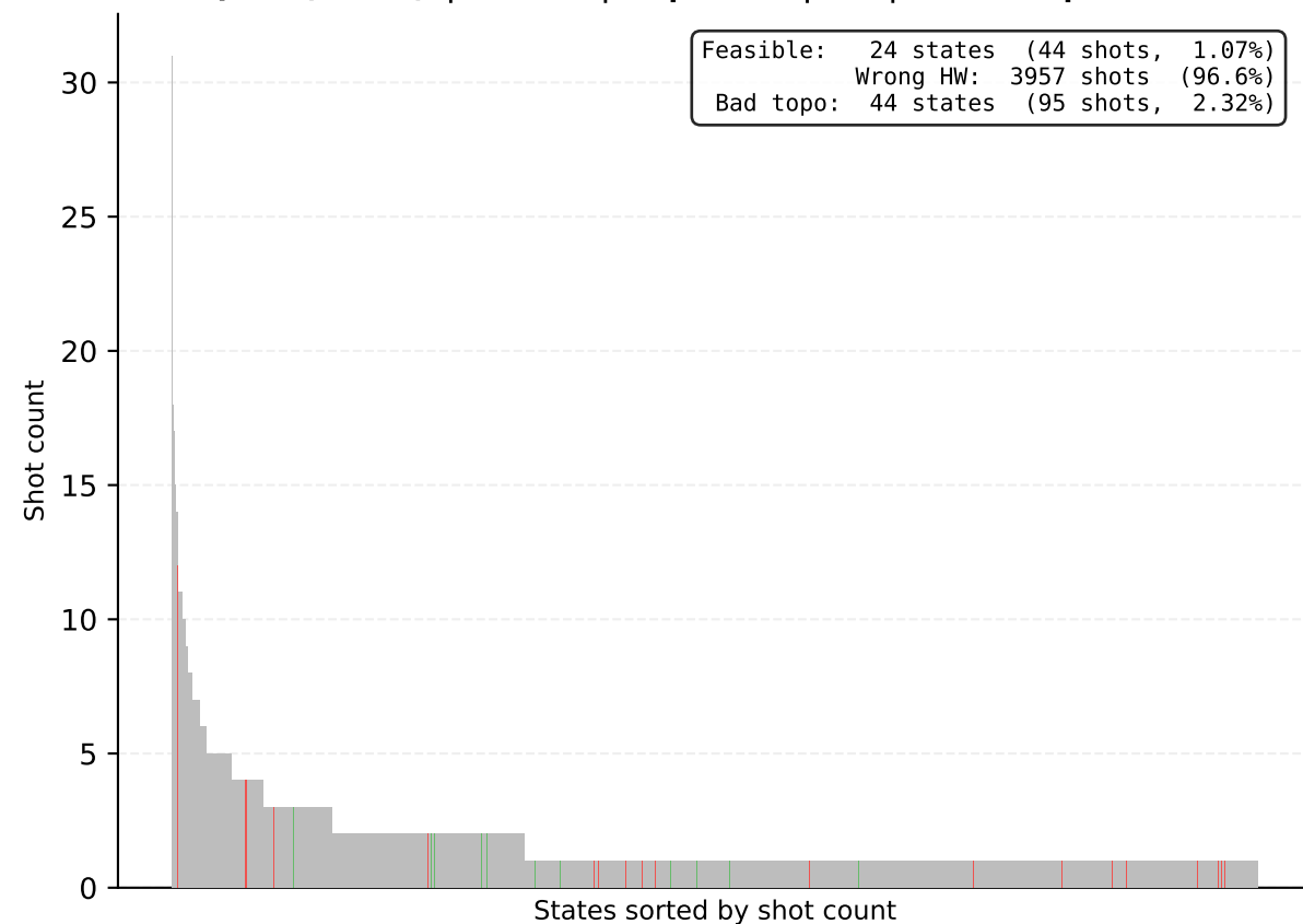
NN-2 QAOA (native) | 15-bus | depth=29 | 1L | 2939 unique / 4096 shots
