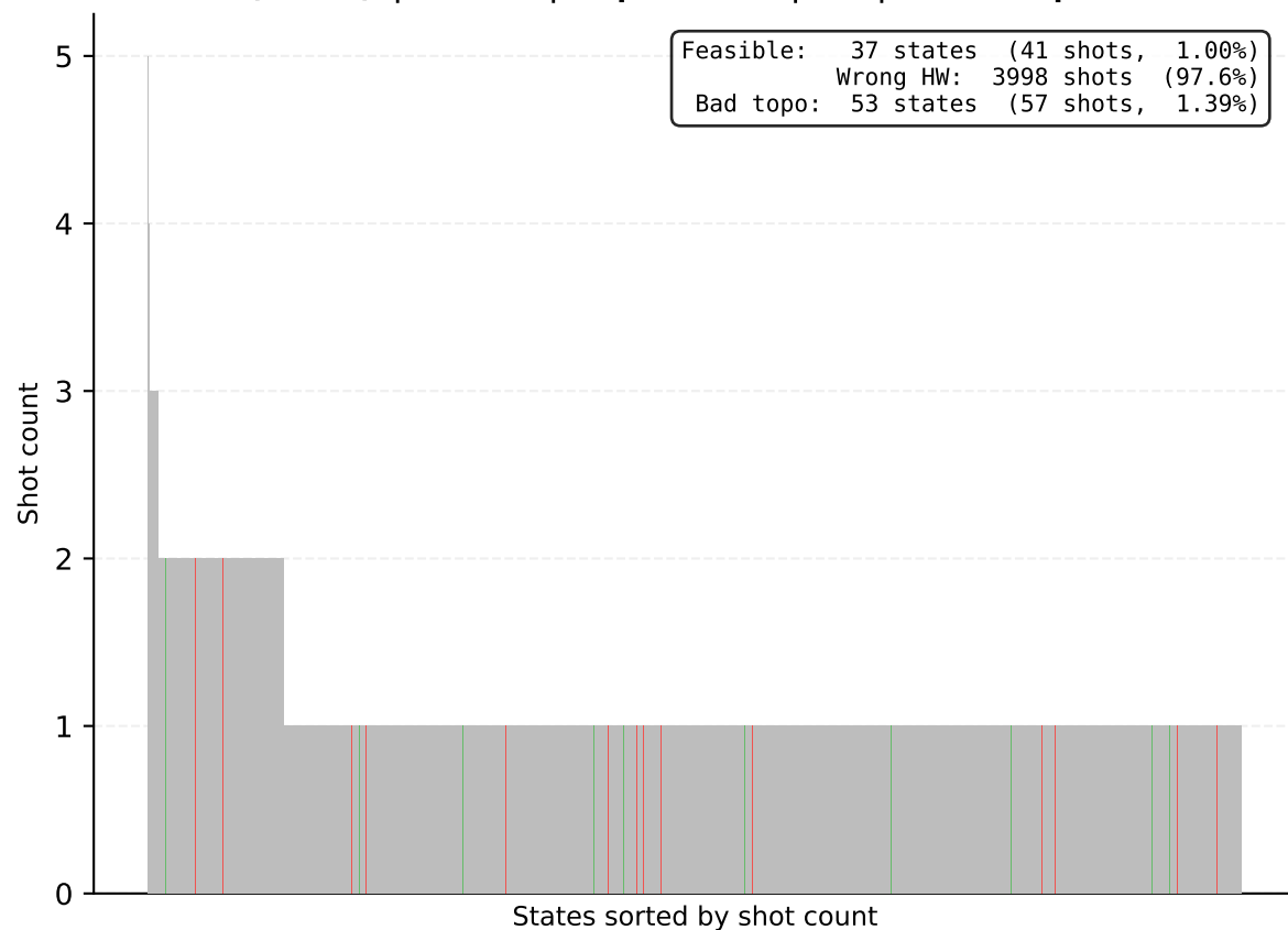
NN-2 AOA (native) | 15-bus | depth=2351 | 1L | 4034 unique / 4096 shots
