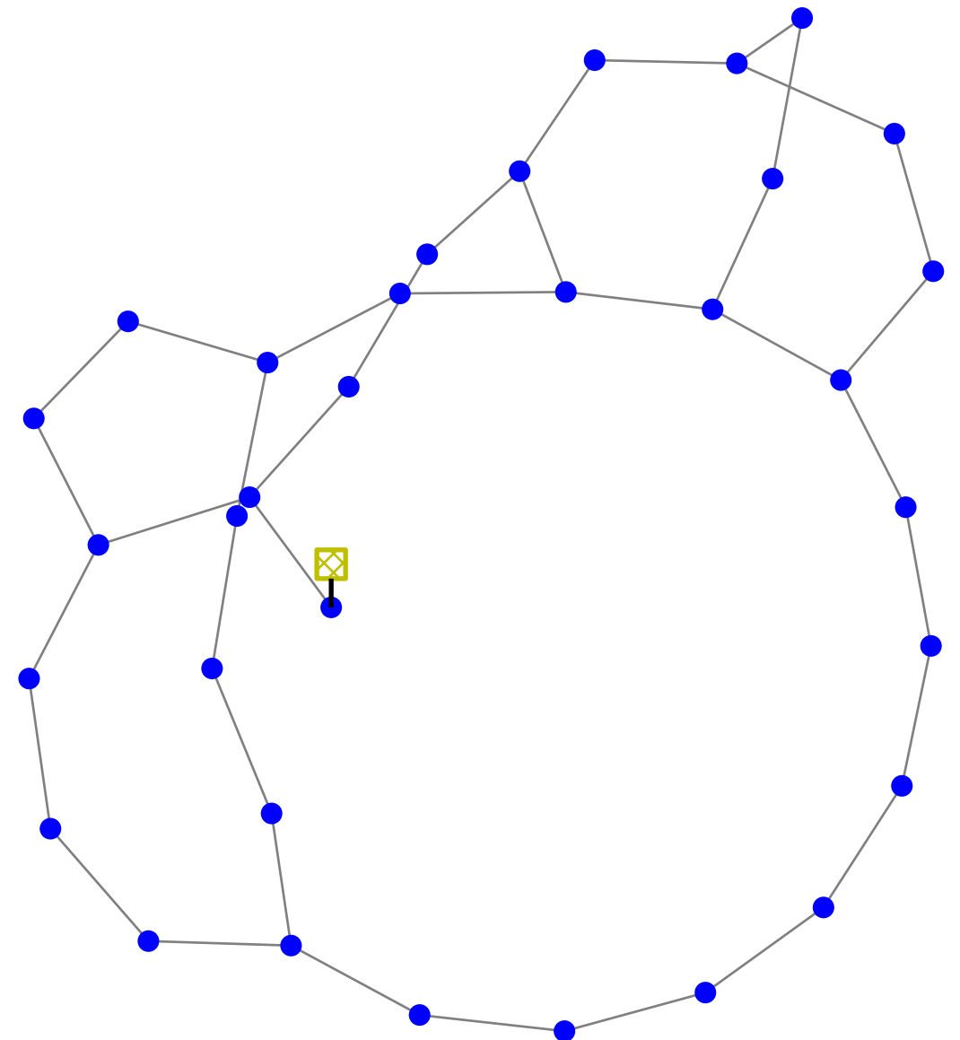
33-bus 33 buses • 37 switches (32 closed, 5 tie)
