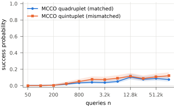
E3: rules of length 4 only (e3/L/R5/0)
