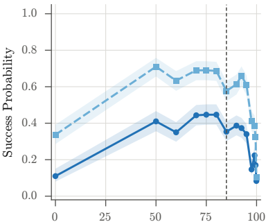
Local Rules
