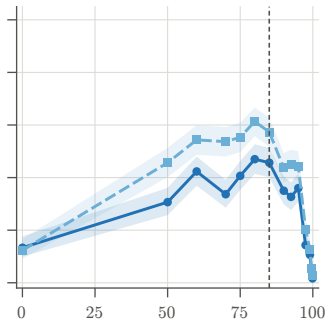
Non-local Rules
