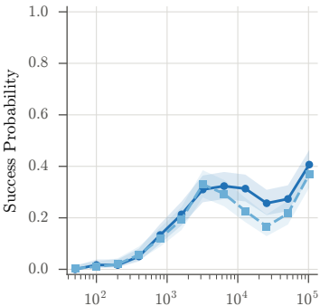
(a) Success
