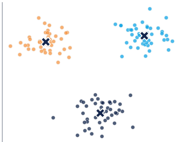
Clusters K-means (k=3)
