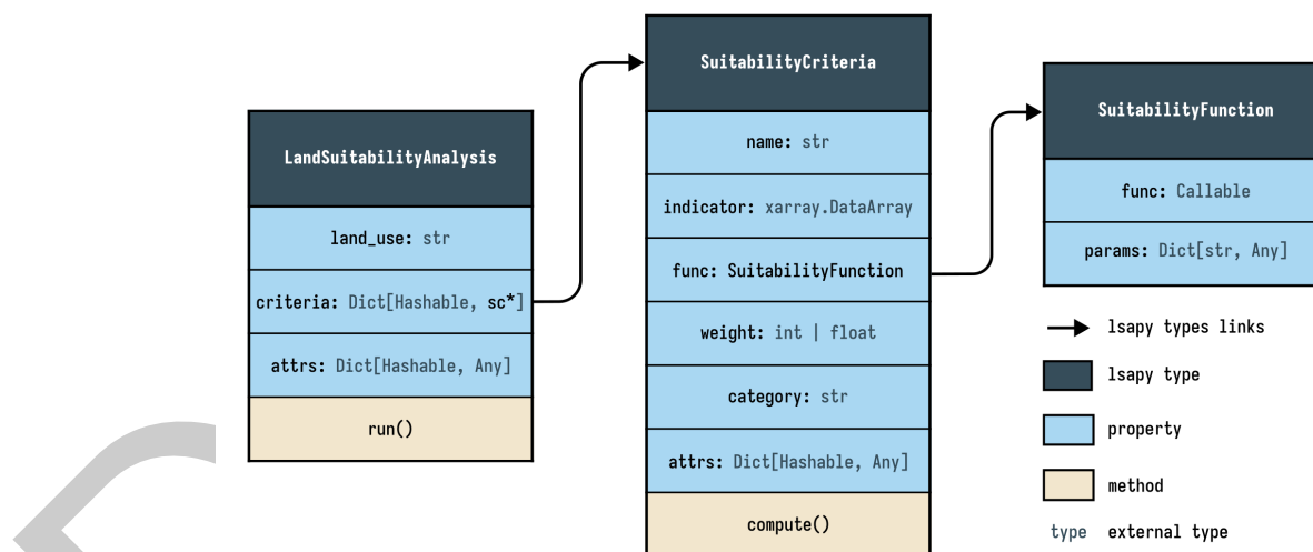
Figure 1: Overview of LSAPy's object structures and their associated properties and methods. *sc is used as an abbreviation of SuitabilityCriteria.
