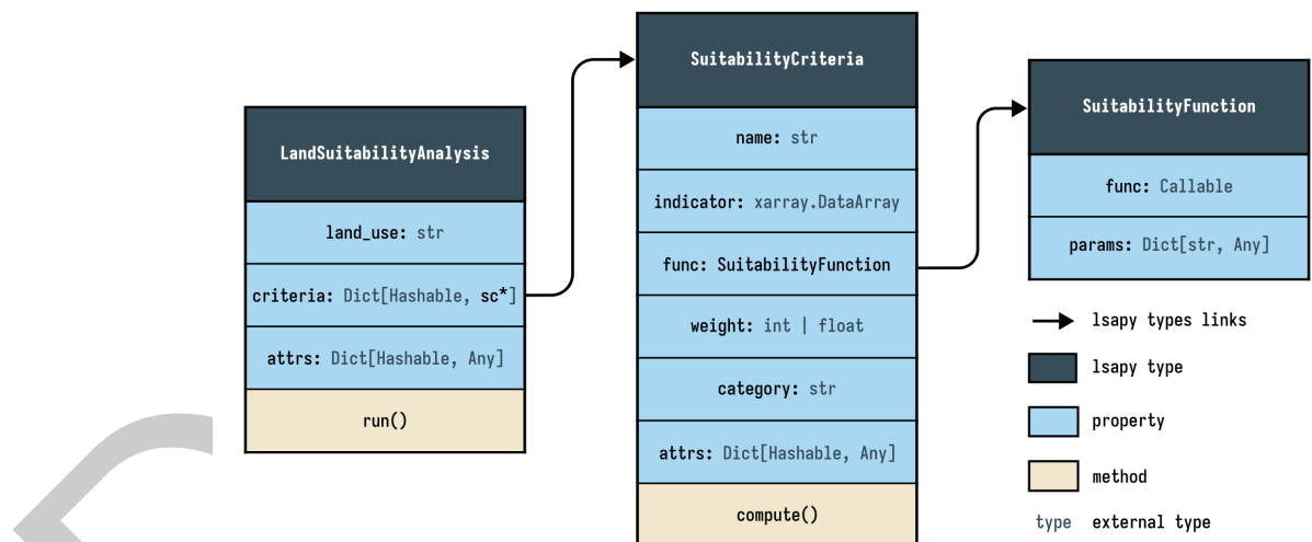
Figure 1: Overview of LSAPy's object structures and their associated properties and methods. *sc is used as an abbreviation of SuitabilityCriteria.
